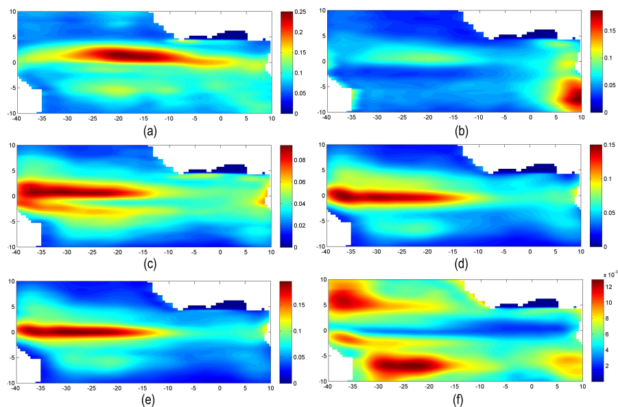
Figure 5: Maps of the standard deviations of TIW anomaly fields of temperature in °C (a), salinity (b), zonal, meridional and vertical velocity components in m/s (c, d and e, respectively) and sea surface elevation in m (f).
