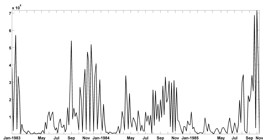
Figure 6: Time series of TIW EKE at 0.25°N/28.25°W, averaged on 5 meters depth (first vertical model layer), extracted from the SODA 5-day mean. The units are \text{ergs/cm}^3 .
