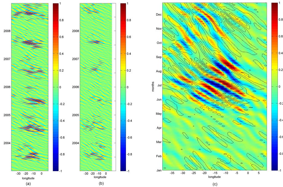
05 Figure 3: Time-longitude plots of filtered sea surface temperature (°C) at 0.25°N. (a) daily TMI; (b) 5-day mean SODA; (c) daily TMI (color) and 5-day mean SODA (black contour) superposition for 2003.
