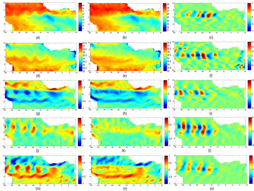
Figure 4: Maps of the total and basic state and TIW anomaly fields (left, middle and right panels, respectively) from the SODA results in the first vertical model layer from August 12 to 17, 2006. (a), 10 (b) and (c) The temperatures in °C; (d), (e) and (f) salinity; (g), (h) and (i) zonal velocity; (j), (k) and (l) meridional velocity; (m), (n) and (o) vertical velocity (m/s).
