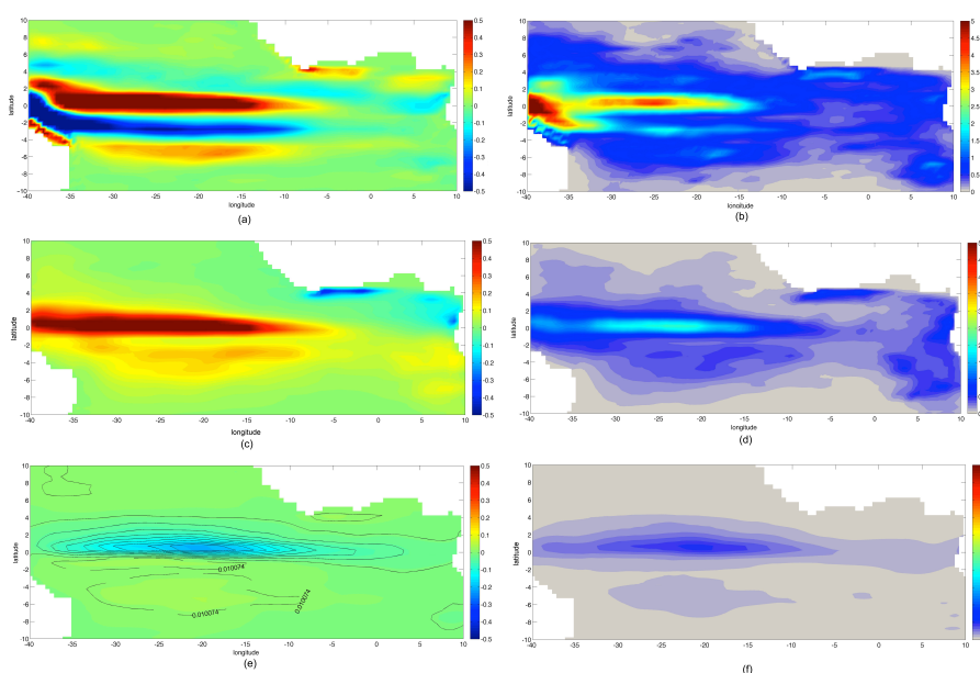
Figure 10: Maps of time mean (a) and standard deviations (b) of barotropic energy conversion rates, time-mean (c) and standard deviations (d) of Kelvin-Helmholtz energy conversion rates and time-mean (e) and standard deviations (f) of baroclinic energy conversion rates. The units are in W/m^3 .
