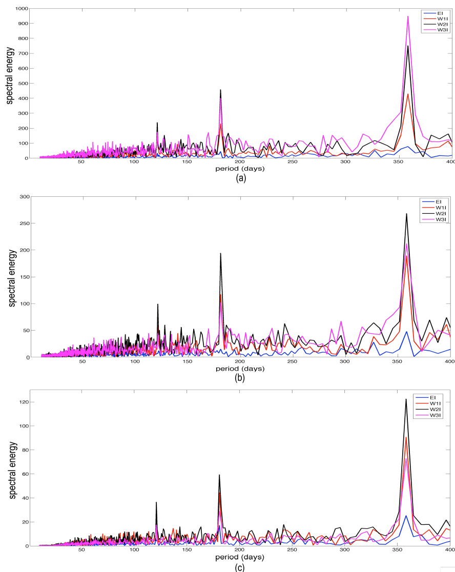
Figure 11: Energy spectra for the index time series of barotropic (a), Kelvin-Helmholtz (b) and baroclinic (c) energy conversions. Blue line is East Index, red line is West 1 Index, black line is West 2 Index and magenta line is West 3 Index. The units are in \text{W/m}^3/\text{day} .
