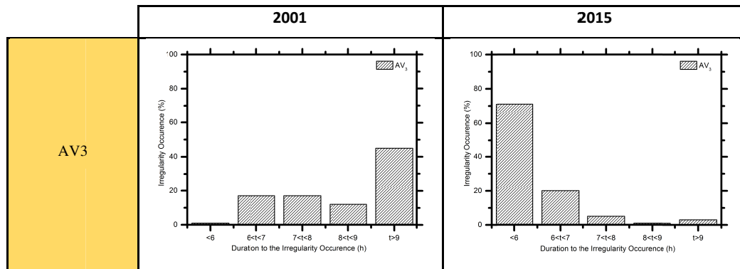
10 FIGURE 3 – Occurrence of spread-F in ionograms for AV 3 index in 2001 and 2015 over São Luís to evidence the differences between the solar flux levels.
