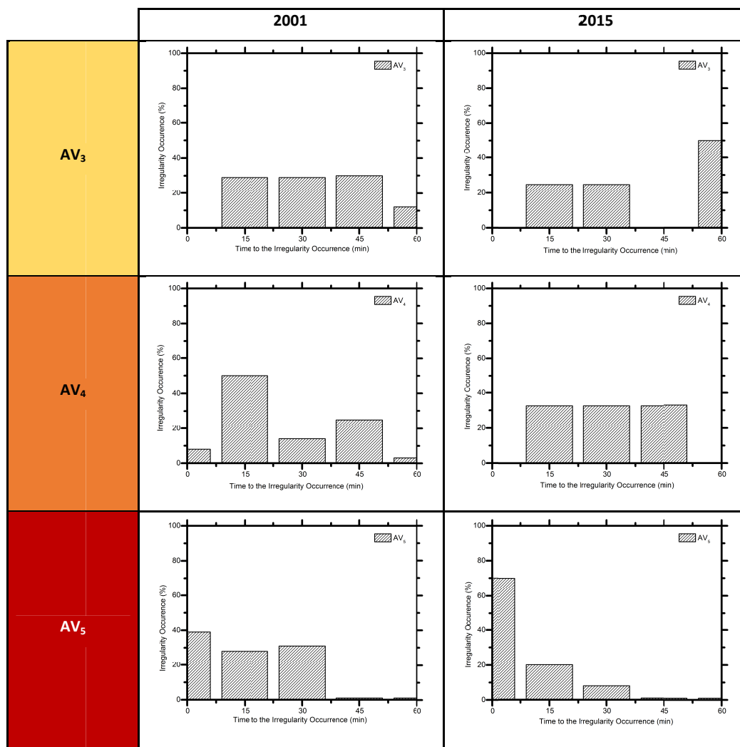
FIGURE 2 – Time relation between the V_{zp} parameter, considering AV_3 , AV_4 and AV_5 indexes, and the irregularity observations in ionograms in the summer of 2001 and 2015 over São Luís.
