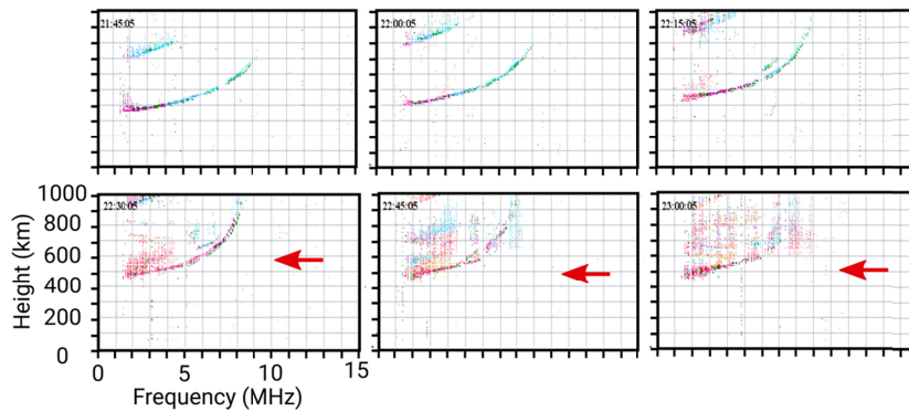
15 FIGURE 1 – Sequences of ionograms showing the spread-F over São Luís on January 26, 2001 (red arrows).
