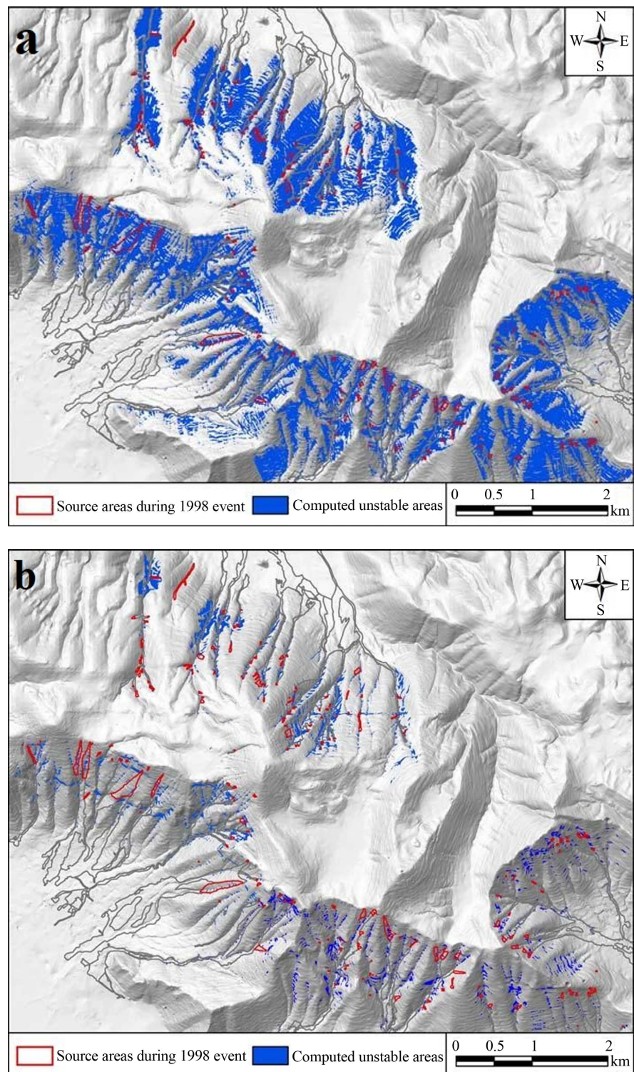
Figure 3. Instability results of Pizzo d'Alvano area from (a) Shalstab and (b) TRIGRS. Source: [43].
