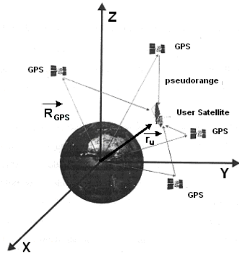
Fig. 2 - Geometric Method for GPS positioning.
