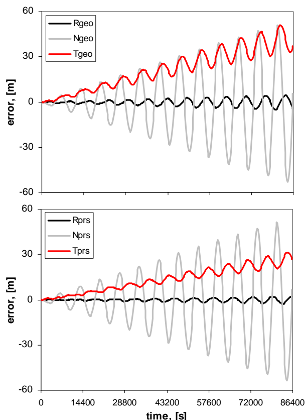
Fig.5 - Orbit propagation per 24 hours period for 11/18/93.
