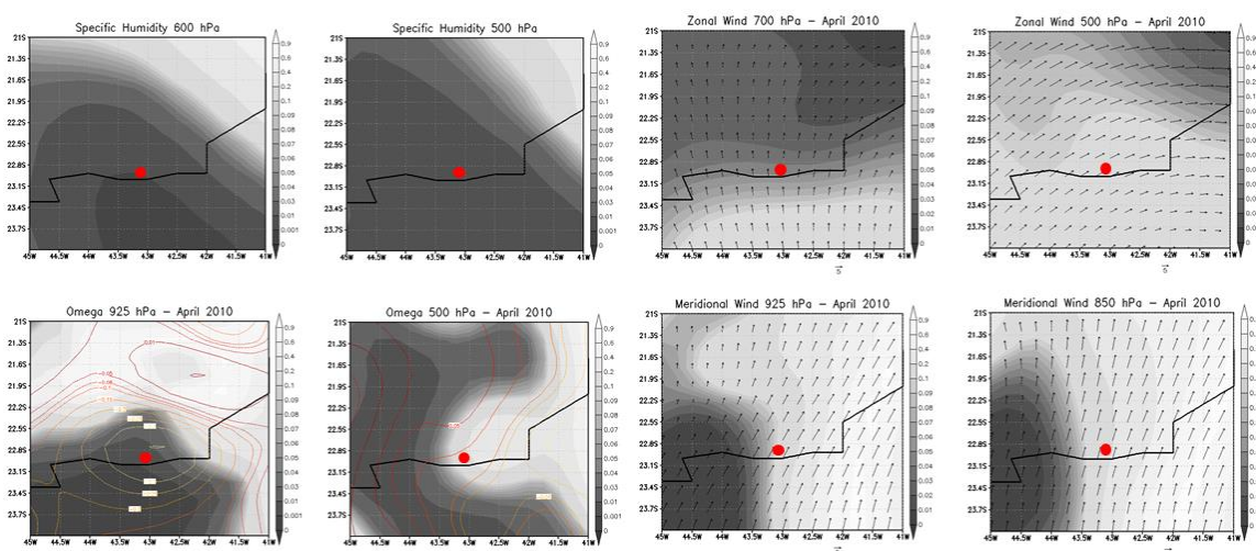
Figure 2. - REPRESENTATION in p-values of the climatic variable influence Specific Humidity (600 and 500 hPa), Omega (925 and 500hPa), zonal wind (700 and 500 hPa), and meridional wind (925 and 850 hPa) in Rio de Janeiro flood .
