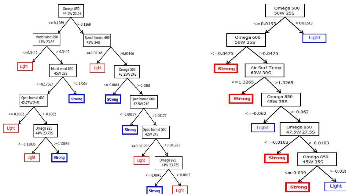
Figure 3: DECISION tree generated: SC flood (right) training set from 2000 up to 2006; test set: 1999, 2007-2010. RJ flood (left) training set from 2000 up to 2006, and test set: from 2007 up to 2010.
