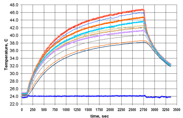
Fig. 8. Start-up with permanent overshoot; heat load is 20W, inclination is +1.5 deg..
