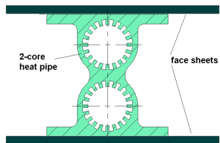
Fig. 1. Two-core heat pipe inserted into honeycomb panel
