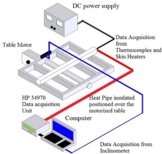
Fig. 2. Experimental setup.
