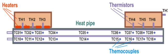
Fig. 3. HP instrumentation.
