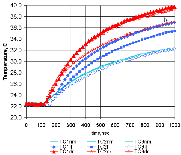
Fig. 13. Superposition of temperature rise in evaporation zone in cases of nominal start-up, overshoot due to dry-out and overshoot due to flooding.
