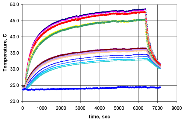
Fig.9. Dry-out under unfavorable inclination of -2 degree 15 W.
