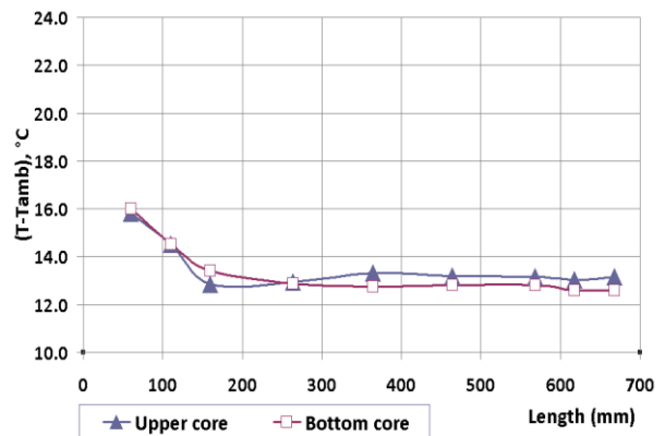
Fig.4. Distortion of the temperature profile under favorable inclination of +2 degrees and heating power of 15 W (trapped slug).
