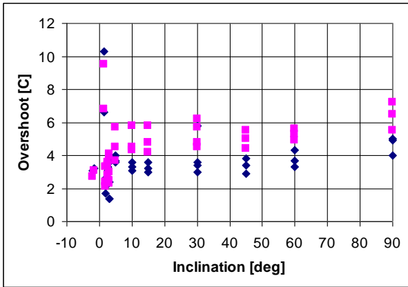
Fig. 12. Temperature overshoots summary.
