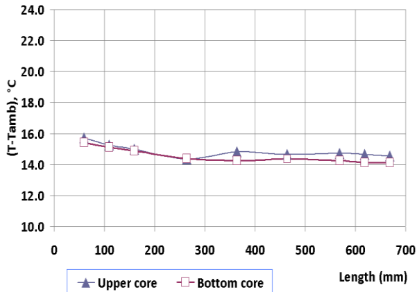
Fig. 5. High equivalent conductance of the HP under unfavorable inclination of -2 degree and 15W.
