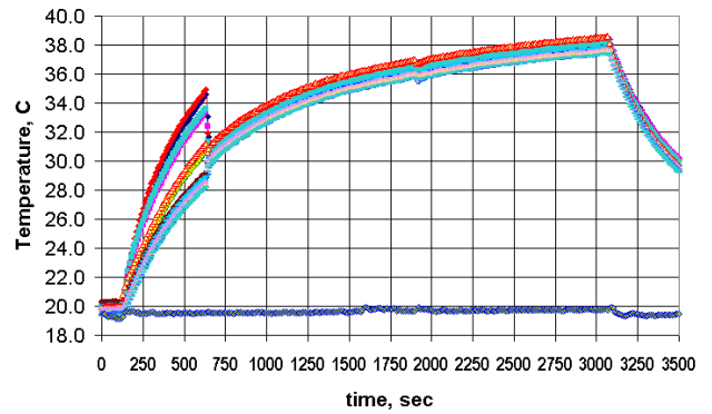
Fig. 7. Start-up with overshoot and delay of 630 sec; heat load is 20W, inclination is +2.5 deg..
