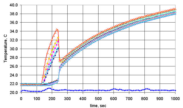
Fig. 11. Temperature overshoot during start-up of the HP at vertical position (25W, 90 deg).
