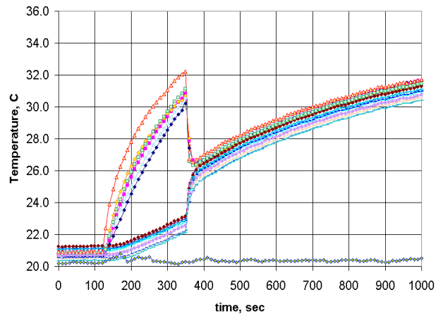
Fig. 10. Temperature overshoot during start-up of the heat pipe at vertical position (15W, 90 deg).
