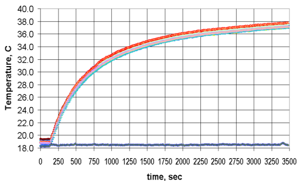
Fig. 6. Smooth nominal start-up, heat load is 20W, inclination is +0.3 deg..
