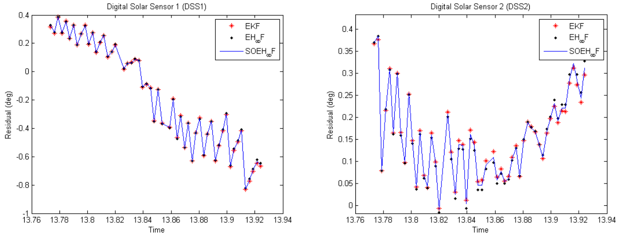
Figure 10. Residuals of the two DSS on board the CBERS-2 satellite
