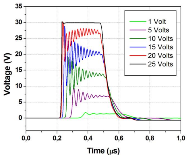
Fig. 18. Corresponding Spice simulations of the pump pulse amplitude effect on the output oscillations.
