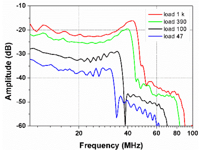
Fig. 14. Spice FFT spectra of the NLTL output pulse obtained for all loads.
