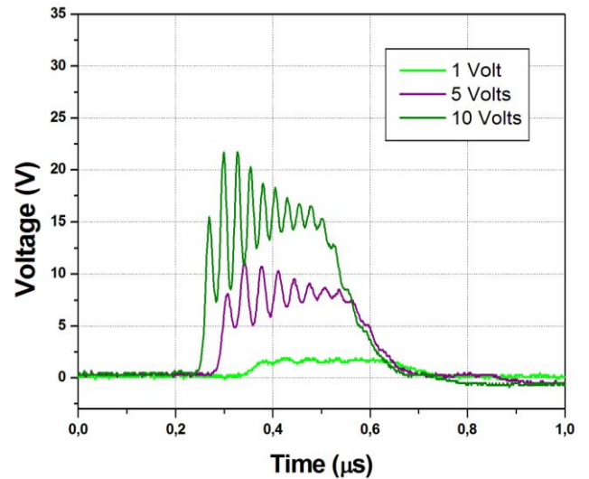
Fig. 17. Effect of the pump pulse amplitude on the output oscillations.
