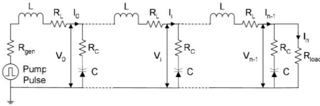
Fig. 5. NLTL schematic circuit used for NLTL simulation using BB809 varactor diodes.
