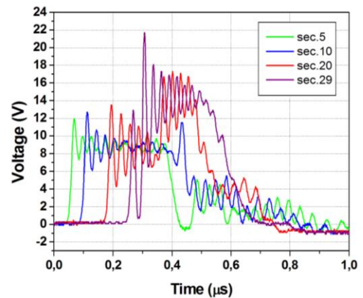
Fig. 8. Experimental voltage pulse obtained for the NLTL on different sections.
