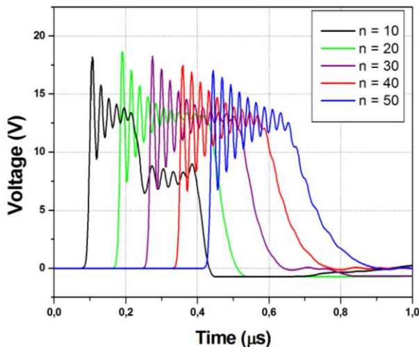
Fig. 16. Corresponding Spice simulation on the load with n increase up to 50.
