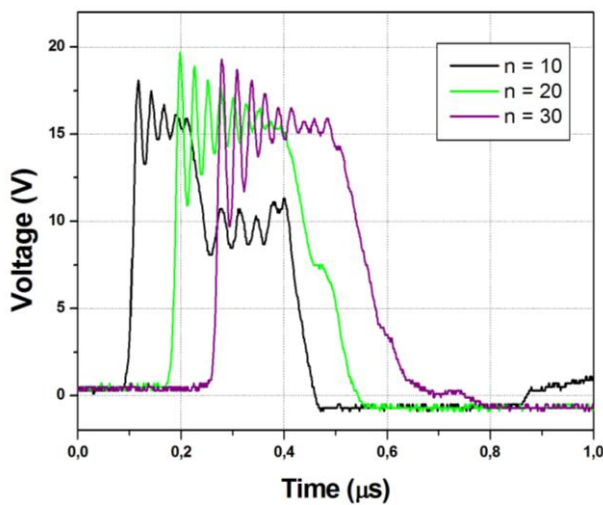
Fig. 15. Effect of the NLTL n increase on the output pulse on the load (last section).
