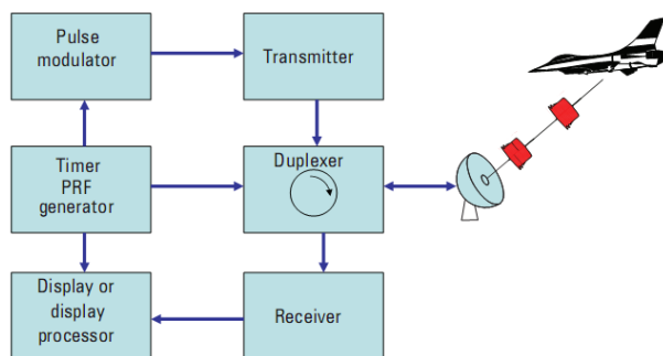
Fig. 1. Block diagram of a basic radar system [1].
