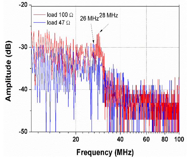
Fig. 12. FFT spectra of the NLTL output pulse with loads of 47 and 100 ohms.
