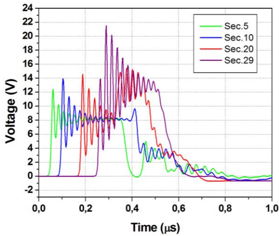
Fig. 9. Corresponding Spice simulation obtained for the NLTL on different sections.
