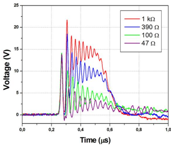
Fig. 10. Variation effect of load resistance on NLTL section 29.
