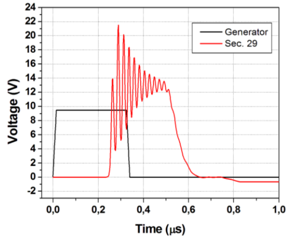
Fig. 7. NLTL simulation pulse voltage on section 29.
