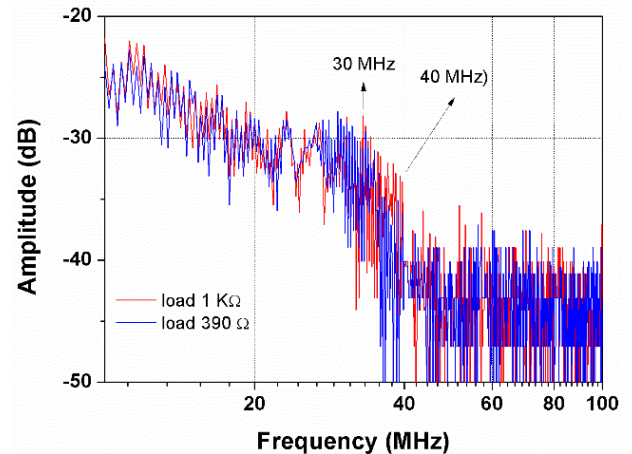
Fig. 13. FFT spectra of the NLTL output pulse with loads of 390 and 1 k ohms.
