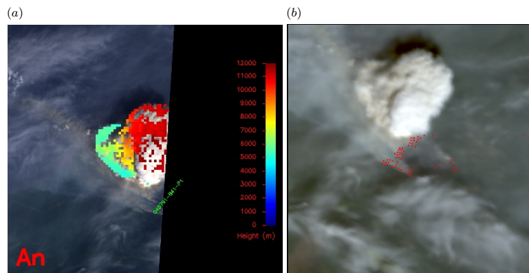
Figure 11. Overview of the highest fire plumes present in the current North American subset of the MISR plume height dataset of Nelson et al. (2008), derived using the MINX tool shown in Figure 4. The reference of this fire in the MISR data set is O45791-B41-P1, and it was observed in the Northwest Territories (Canada) on 27 July 2008. (a) shows the nadir image recorded by MISR, together with the stereo-height retrieval of the MINX model. Part of the image is black as the fire was located on the edge of the MISR swath. (b) is the wider-swath Moderate Resolution Imaging Spectroradiometer (MODIS) false color composite image of the area observed at the same time. MODIS is mounted on the same Terra satellite as MISR (see Sect. 4.1). Red pixels denote the location of MODIS pixels detected as containing active fire in the MODIS MOD14 active fire product of (Giglio et al., 2003). Image (a) is taken from the MISR plume height project website (see Footnote 1).
