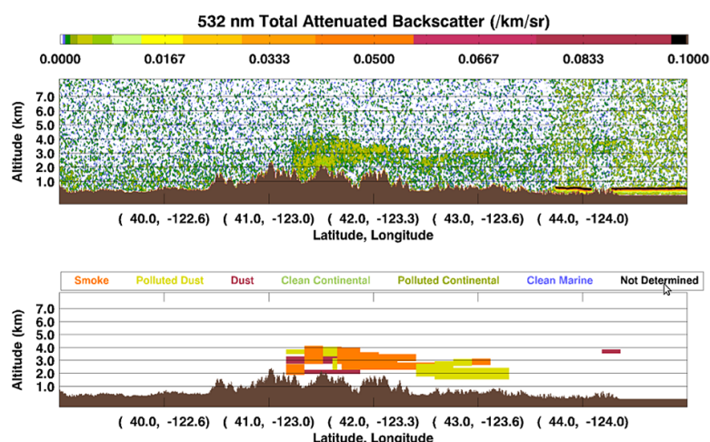
Figure 3. Example of profiles for Level-1 CALIOP 532 nm total attenuated backscatter data product (top), and the matching level-2 product of aerosol layers (bottom) for the 28 August 2006 over the Klamath mountains in California and Oregon. The presence of aerosols classified as biomass burning smoke can be seen. Image from Raffuse et al. (2012).
