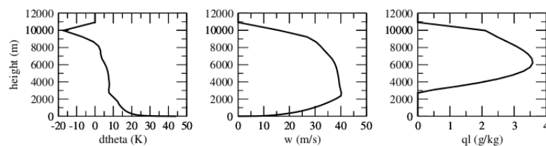
Figure 6. Smoke plume characteristics for the Chisholm fire, as simulated by pyro-EDMF: virtual potential temperature (K), vertical velocity excess ( \text{m s}^{-1} ), and cloud liquid water ( \text{g kg}^{-1} ) are shown. Figure from Rio et al. (2010).
