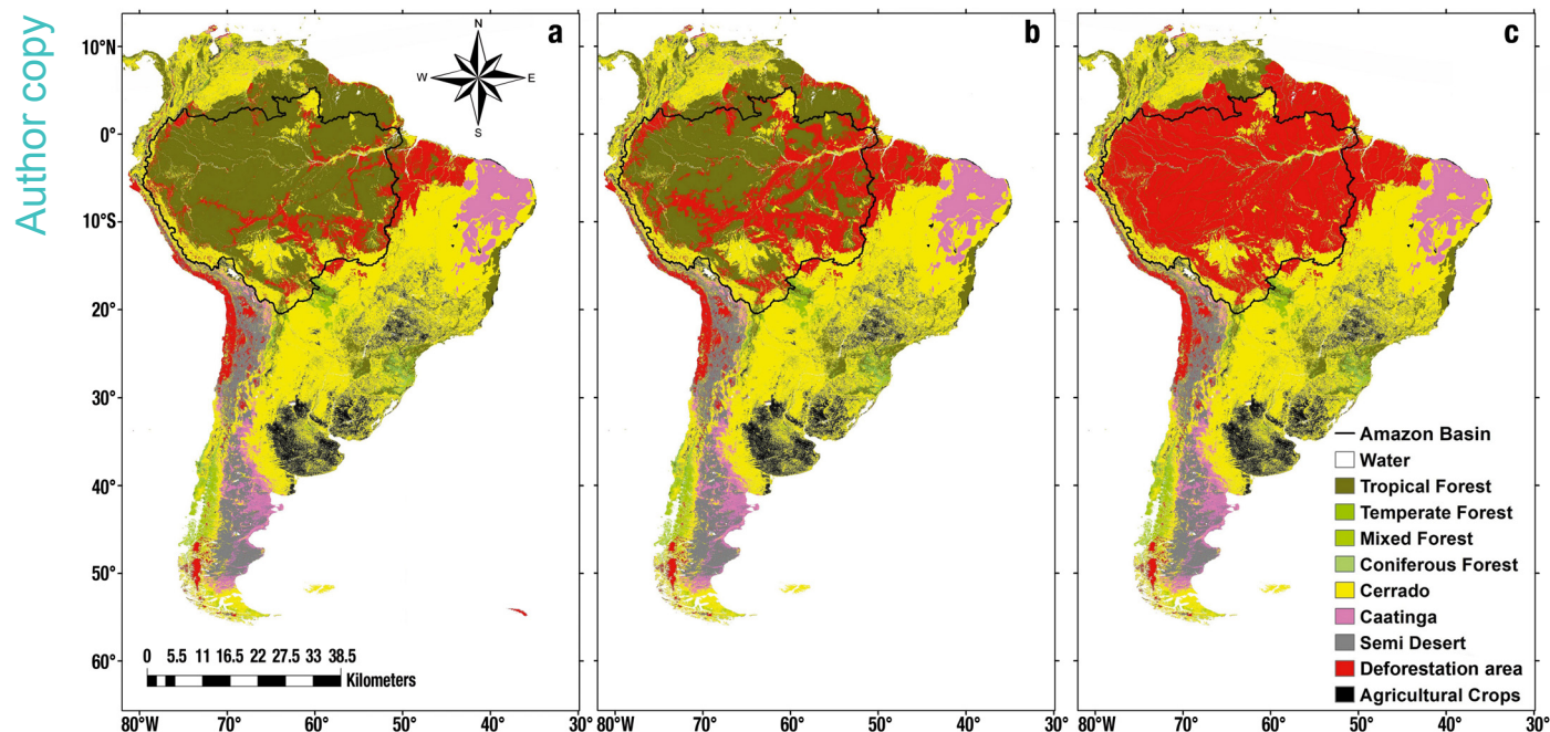
Fig. 1. Vegetation cover scenarios used in simulations with the Eta regional model. (a) Vegetation map prepared by the ProVeg Project with deforested areas (base year 2015); and scenarios projected for the year (b) 2050 and (c) 2100. Both scenarios elaborated by the DINAMICA model. Resolution: 1 \times 1 km
