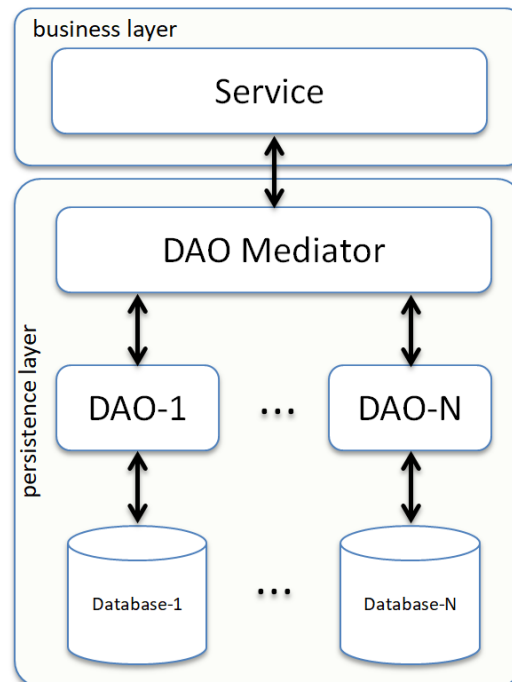
Fig. 3. DAO Compound Mediator Pattern Scheme.
