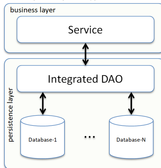
Fig. 2. Integrated Polyglot DAO Pattern.
