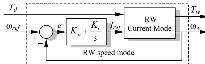
Figure 3: Reaction Wheel speed control loop.
