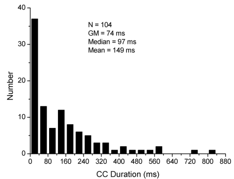
Figure 3. Histogram of the CC durations in 104 positive strokes.
