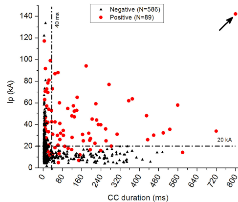
Figure 4. Scatterplot of the estimated peak current, I_p , versus CC duration.
