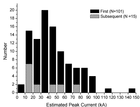
Figure 2. Histogram of the estimated peak currents in positive first and subsequent strokes.
