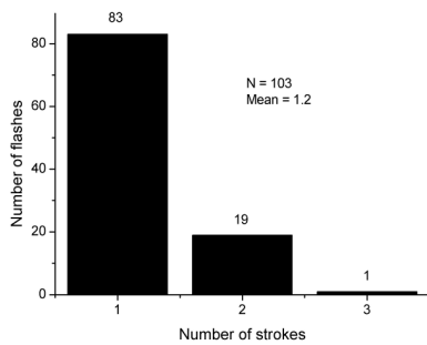
Figure 1. Number of flashes that contained the given number of strokes. The total number of strokes was 124.
