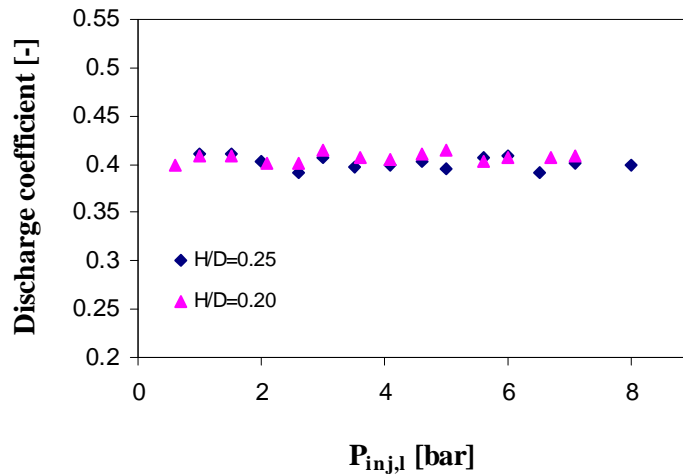
Figure 4. Discharge coefficient of the blurry injector without gas flow.
