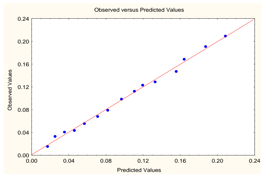
Figure 10. Correlation between predicted values by regression nonlinear and observed values for H/D = 0.25 .
