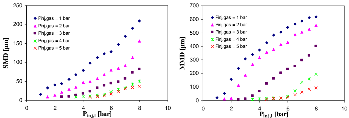
Figure 8. Experimental Sauter mean diameter (SMD) and mass median diameter (MMD) for H/D = 0.25 .
