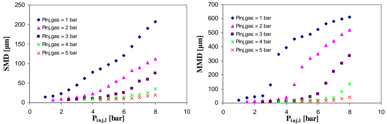
Figure 7. Experimental Sauter mean diameter (SMD) and mass median diameter (MMD) for H/D = 0.20 .
