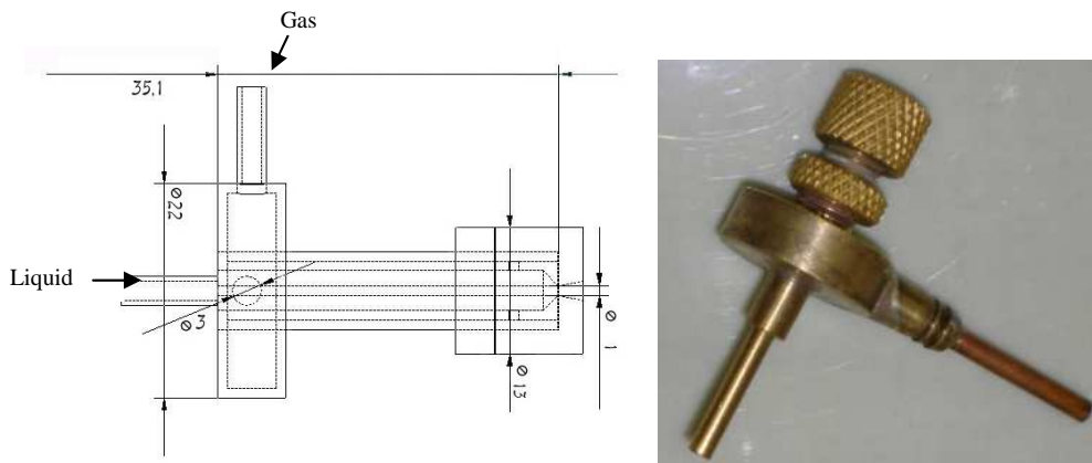
Figure 2. Schematic representation and photo of the Blurry injector.
