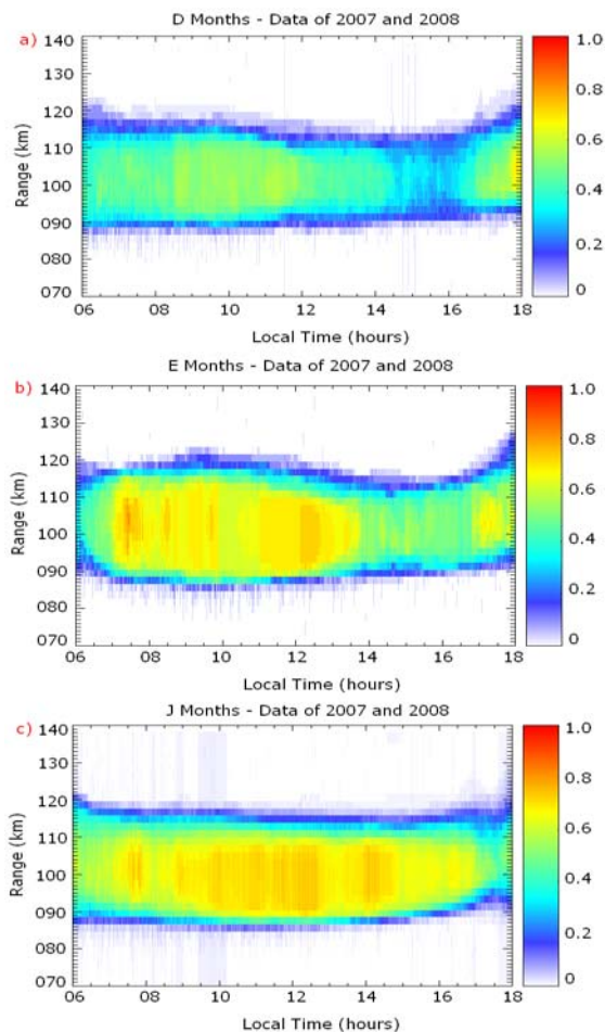
FIGURE 6: Statistical RTI map of JULIA. (a) is the summer, (b) is the equinoxes months and (c) is the winter.
