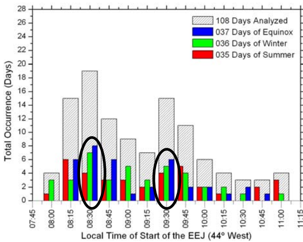
FIGURE 2: Histogram of days of occurrence versus the begin hour of the irregularities observation in the EEJ, with data RESCO.
