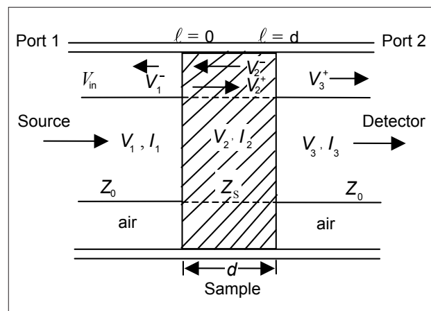
Figure 1: Waveguide filled with material. ( Z_0 is the impedance of air, Z_s is the impedance of the material, V_n ( n = 1, 2, 3 \dots ) is the voltage, I_n ( n = 1, 2, 3 \dots ) is the intensity, n is the interface between the means, d is the sample thickness and \ell is the thickness of line of air (ASTM, 2001; Nicolson and Ross, 1970).
