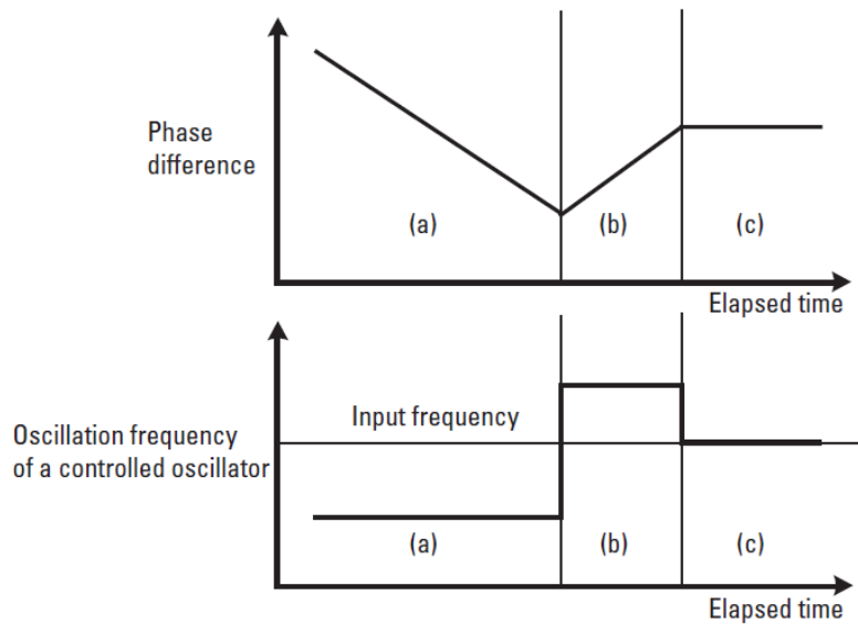
Figure 7. Phase difference and output frequency change over time during a phase synchronization process (digital control): (a) initial condition, (b) condition between the first and second digital controls, and (c) condition after the second control. Source: Kihara et.al (2003).
