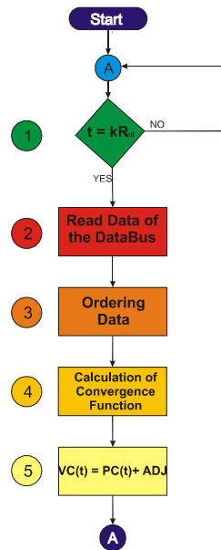
Figure 5. Flowchart of FTM Algorithm.
