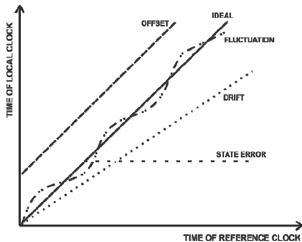
Figure 1. Clock errors.
