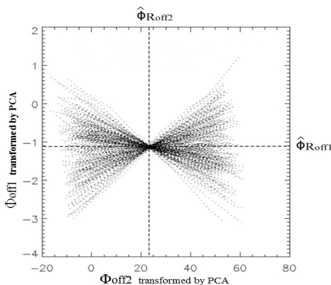
Figure 8. Example of the CPOFs transformed by PCA.
