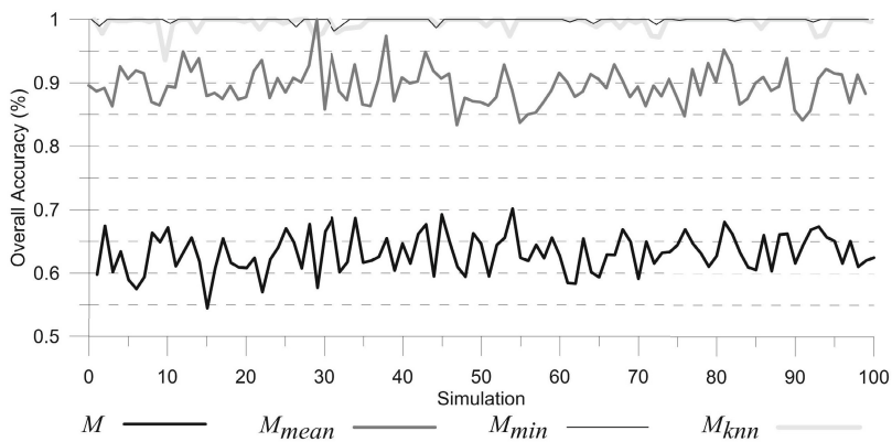
Fig. 3. Overall accuracy results for four classes image
