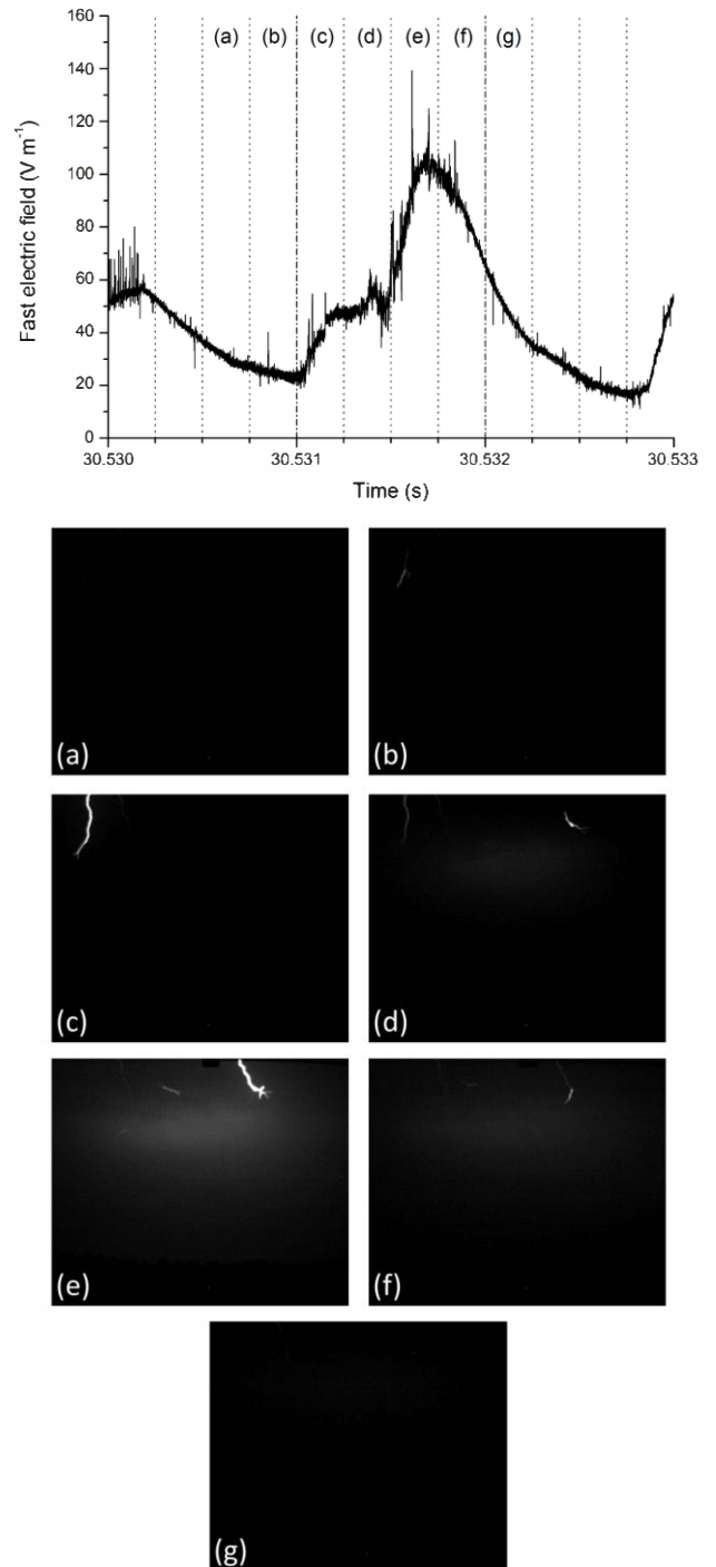
Figure 1. Fast electric field waveforms related to the occurrence of visible recoil leaders (recorded at 4000 frames per second).
