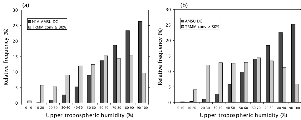
Figure 8. Upper tropospheric humidity (UTH) distributions for cases when AMSU DC (dark gray) or TRMM convective percentage >80% (light gray) were found. UTH is relative to ice; only UTH ≤ 100% were considered. The period considered was October 2002 to April 2003. (a) Distribution using only NOAA-16 satellite data, which overpasses the target region around 0200 and 1400 LT, and (b) distribution using NOAA-15, -16 and -17, covering several hours of the diurnal cycle.
