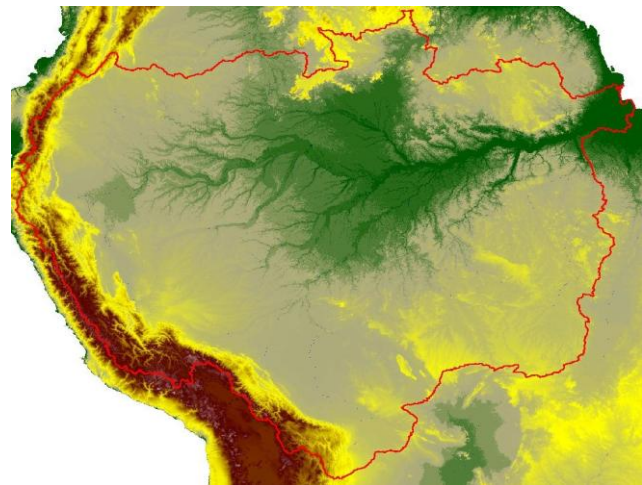
Figure 15 Drainage network of Amazonian basin.
