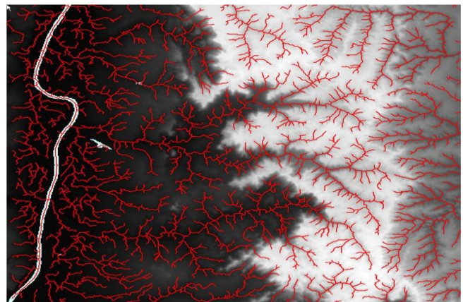
Figure 10 Drainage network of Taquaruçu basin (red color) on a grayscale DEM.
