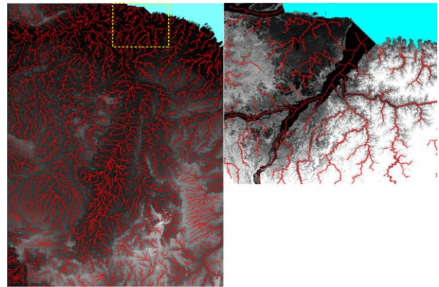
Figure 14 Drainage network of Tocantins basin.
