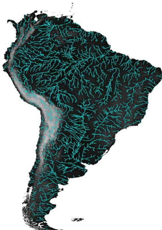
Figure 16 Drainage network of South America region.
