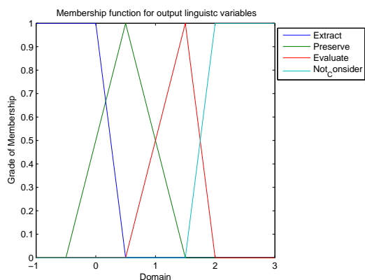
(b) Output linguistic terms.
