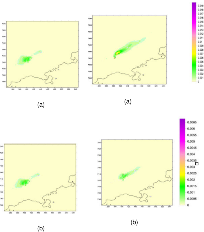
Figure 5: Winter: Output of the model of dispersion of pollutants CALPUFF concentration of CO with spatial resolution of 1 km for the day July 12, 2004 at 12 h (a) and 24 h (b).
