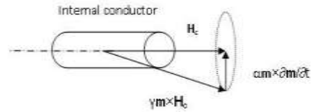
Fig. 4. Mechanism of induced magnetic precession in loaded ferrite lines.
