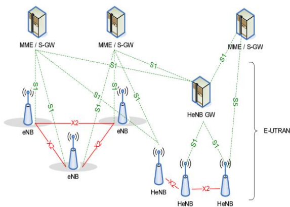
Figure 4. Overall E-UTRAN Architecture with deployed HeNB GW [20]
