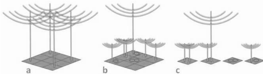
Figure 1. Possible spatial configuration of araucaria trees: (a) Adult trees cannot live in directly neighboring cells. (b) Seeds and juveniles can be in the same cells as other seeds and juveniles and as adults, and in neighboring cells. (c) Possible combinations of individuals in one cell.
