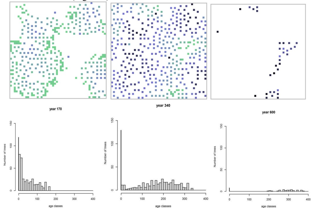
Figure 2. Simulation without disturbance: araucaria population after 170, 340 and 600 years; individual trees color-coded from green (young) to dark violet (old); histograms showing respective age classes.
