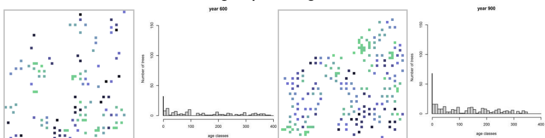
Figure 3. Simulation with fire disturbance: Araucaria population after 600 and 900 years; histograms showing respective age classes.
