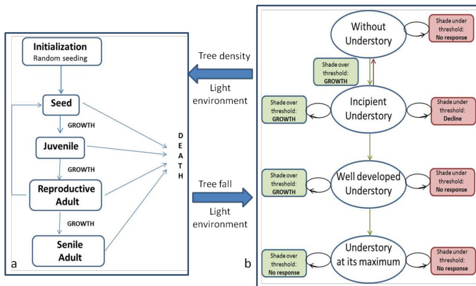
Figure 2. Conceptual model representation and submodels interactions. a) agent module; b) cellular automata module
