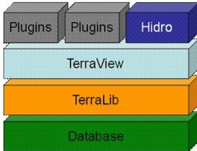
Figure 3.1. - Relationship between Terralib, Terraview and TerraHidro
