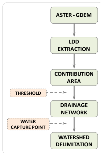
Figure 3.2. TerraHidro tasks sequence to define drainage networks and watersheds.
