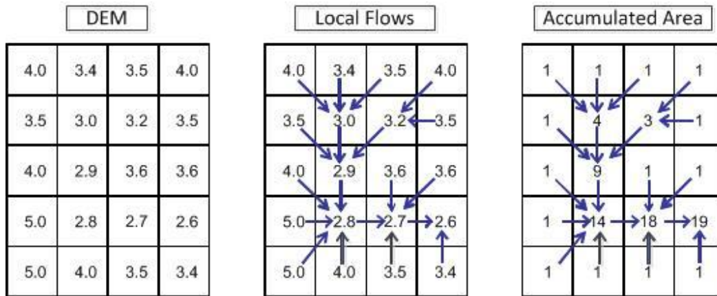
Figure 3.3. Contribution area processes.
