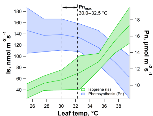
Figure 3. Average net photosynthesis (Pn) and isoprene emissions (Is) from V. guianensis leaves as a function of leaf temperature (average \pm 1 standard deviation, n = 5 leaves) under constant PAR of 1000 \mu\text{mol m}^{-2} \text{s}^{-1} and 400 ppm reference [\text{CO}_2] . Note the decline in Pn and the increase in Is with leaf temperature above 30.0\text{--}32.5^\circ\text{C} , where the majority of leaves showed an optimum in Pn. Pn was determined with a portable photosynthesis system (LI-6400XT, LI-COR Inc., USA) and Is was determined using thermal desorption GC-MS.
