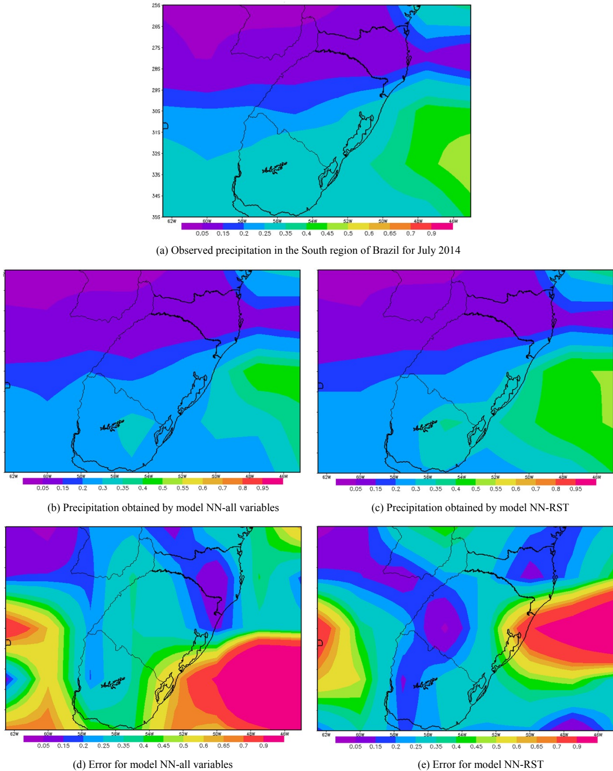
Figure 3. Result for the monthly climate precipitation prediction for the South region of Brazil at July 2014. (a) shows the observed precipitation field extracted from the NCEP/NCAR database; (b) shows the results obtained by NN-all variables, that was design by MPCA, and was trained using all variables available; (c) precipitation obtained with NN-RST trained with a reduced set, and the topology was self-configured by MPCA; (d) shows the difference between observation field and precipitation prediction for model NN-all variables; and (e) error for model NN-RST, trained with a reduced set
