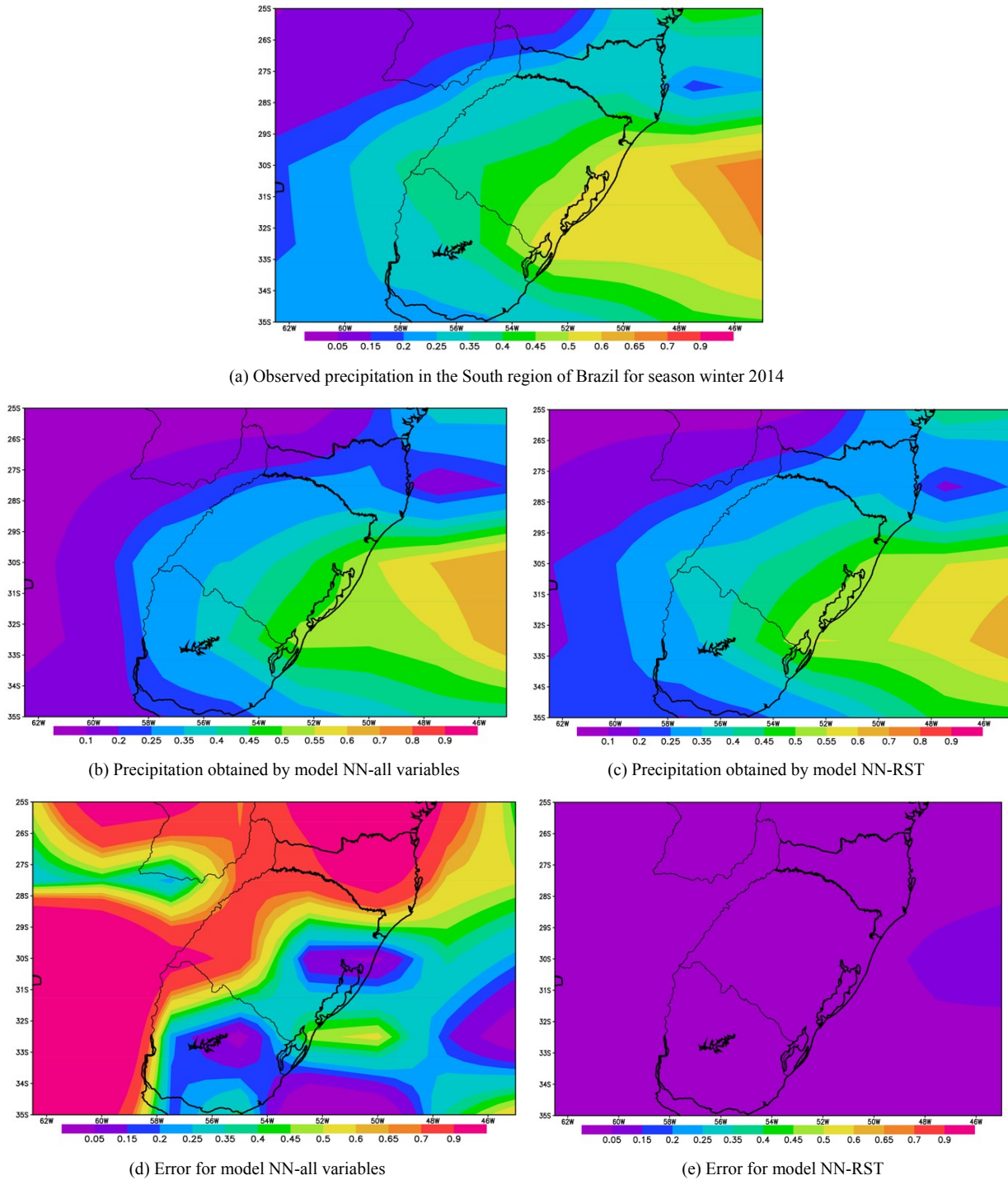
Figure 4. Result for the seasonal climate precipitation prediction for the South region of Brazil in winter 2014. (a) shows the precipitation field extracted from the NCEP/NCAR database; (b) shows the seasonal precipitation result obtained by NN-all variables, that was design by MPCA, and was trained using all variables available; (c) presents the seasonal precipitation obtained by model NN-RST trained with a reduced set, and the topology was self-configured by MPCA; (d) shows the difference between observation field and precipitation prediction for model NN-all variables; and (e) error for model NN-RST, trained with a reduced set
