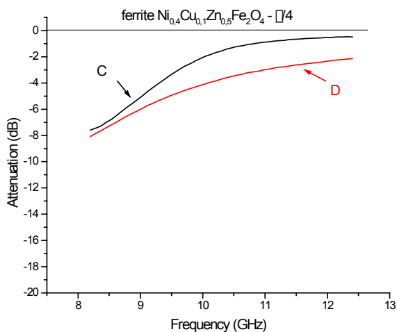
Figure 3 – Reflectivity curves of RAM samples as function of the frequency, prepared with \text{Ni}_{0.4}\text{Cu}_{0.1}\text{Zn}_{0.5}\text{Fe}_2\text{O}_4 ferrite treated at 1000 °C (code C) and 1100 °C (code D).
