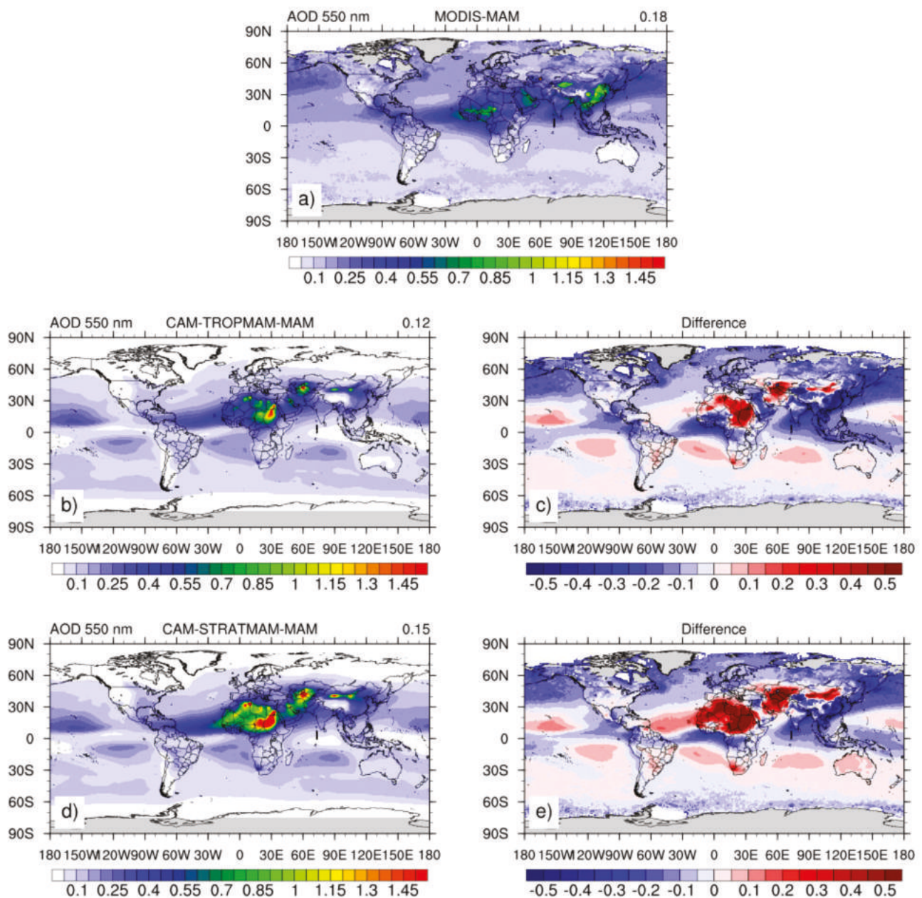
Figure 7. (a) AOD observed by MODIS sensor for March–April–May (MAM), in the period of 2010–2014, (b) AOD simulated by the CAM5-MAM3 model using tropospheric chemistry and (d) tropospheric/stratospheric chemistry mechanisms. The right side of the figure shows the model difference minus the observation (MODIS), (c) for tropospheric chemistry and (e) for tropospheric/stratospheric chemistry.
