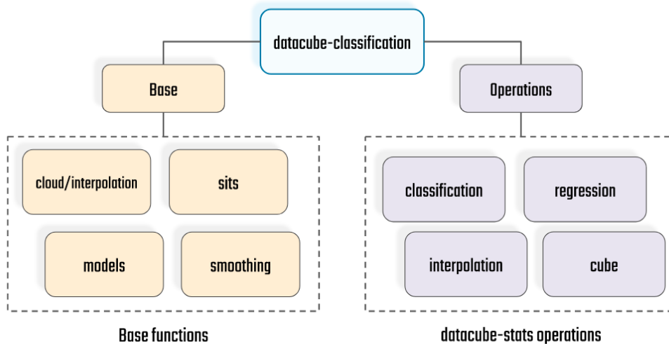
Figure 3 – datacube-classification modules and submodules.
