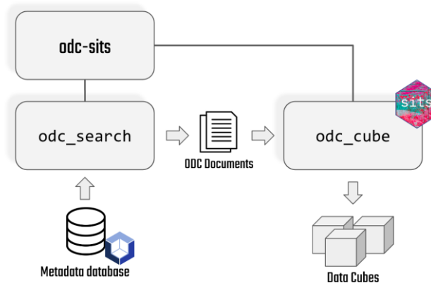
Figure 4 – odc-sits usage process.
