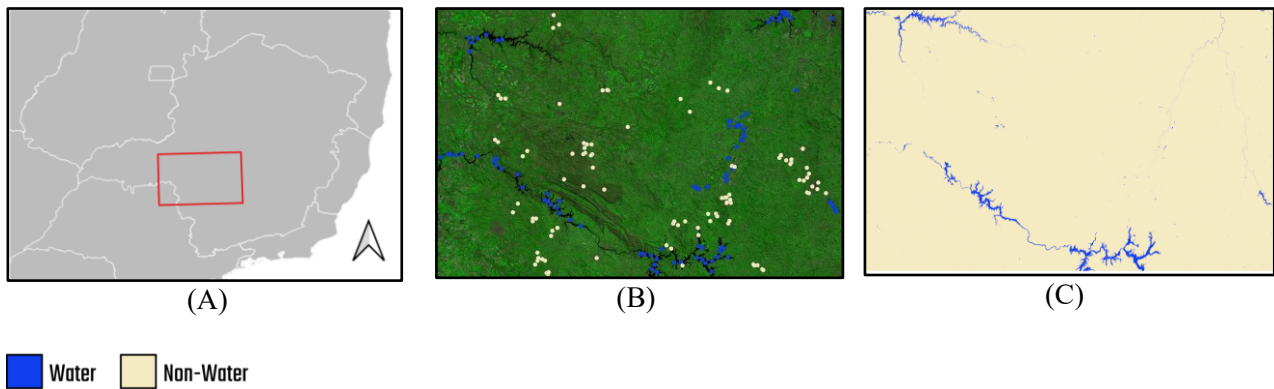
Figure 6 – (A) Study area used for the generation of the water mask; (B) Distribution of the sample set used; (C) Water mask generated with the application of the described methodology.
