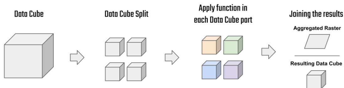
Figure 2 – datacube-stats operation.
