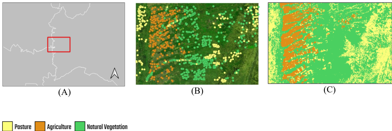
Figure 7 – (A) Study area used for generating the LULC map; (B) Distribution of the sample set used; (C) LULC map generated with the classification process.
