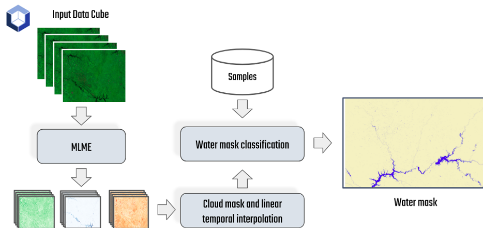
Figure 5 – Methodology for water mask generation.
