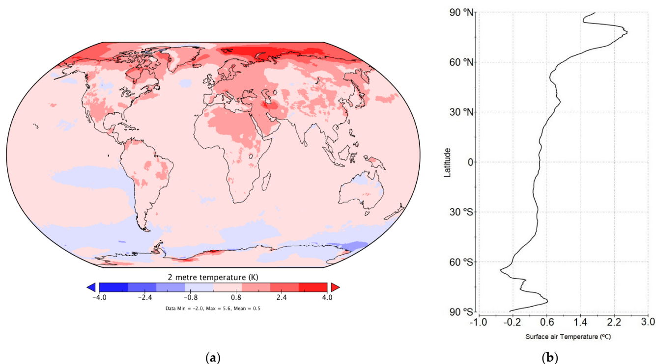
Figure 2. (a) Global map of the polar amplification measure obtained from long-term observations of the near-surface air temperature (°C) for the 2010–2020 period relative to the 1980–1990 period. (b) Zonal mean of the near-surface temperature (°C) for the 2010–2020 period relative to the 1980–1990 period.
