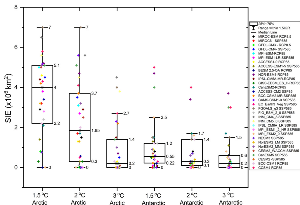
Figure 6. Arctic and Antarctic SIE summer minimum considering the temperature threshold of +1.5 °C, 2.0 °C and 3.0 °C global mean warming under RCP8.5 and SSP585 scenarios. The Arctic's (Antarctica's) summer minimum occurs in September (March).
