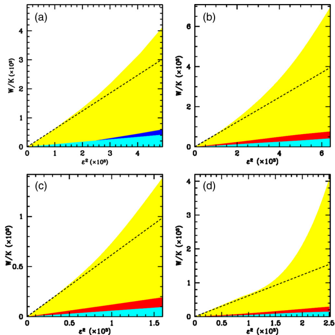
FIG. 15. Phase diagrams for various TT systems. The white, yellow, red, cyan, and blue regions correspond to the commensurate, striped, twisted 2D moiré, 2D moiré, and zigzag phases, respectively. The dashed line corresponds to the sine-Gordon prediction for the stripe-commensurate transition. See text for details. (a) 1 \times 1 ; (b) \sqrt{3} \times \sqrt{3} R30^\circ ; (c) 2 \times 2 ; and (d) \sqrt{7} \times \sqrt{7} R19.1^\circ .
