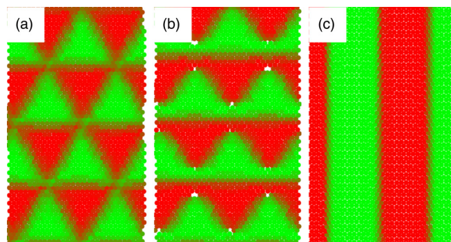
FIG. 16. Sample configurations for the TT (1 \times 1) system showing 2D moiré, zigzag and striped phases in (a), (b), and (c), respectively at \epsilon = 7\% . Here W/K = 0.399 \times 10^{-3} , 0.599 \times 10^{-3} , and 4.051 \times 10^{-3} in (a), (b), and (c), respectively.
