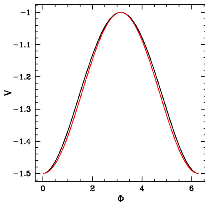
FIG. 8. The figure shows the exact potential Eq. (30) (black line) compared to the approximate solution given in Eq. (31) (red line).
