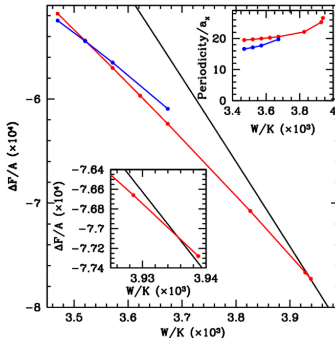
FIG. 12. Free-energy density difference from an incommensurate ( W/K = 0 ) state as a function of W/K for 2D moiré (blue), striped (red), and commensurate (black) phases at \varepsilon = 8\% . In the bottom left inset is a blowup showing that the free energy of the stripes becomes higher than that of the commensurate phase indicating a discontinuous phase transition. In the top inset the periodicity of the 2D moiré (blue) and striped (red) states is shown.
