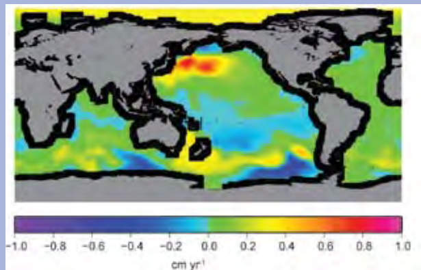
FIG. 2.32. Mean rate of change of ocean bottom pressure (cm yr -1 in equivalent sea level) from January 2003 to August 2010, computed from GRACE data projected onto empirical orthogonal functions (EOF) modes from a model (Chambers and Willis 2008). The large trends in the North Pacific, South Pacific, and Arctic are related to changing circulation and wind stress, and have been described by Chambers and Willis (2008), Boening et al. (2011), and Morison et al. (2007), respectively.
