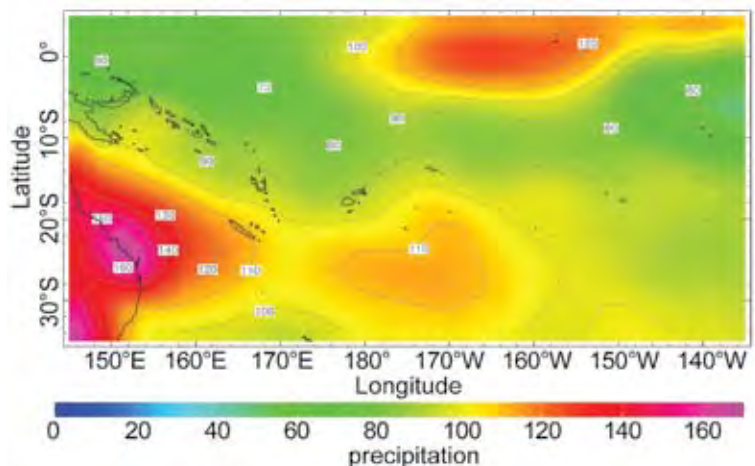
FIG. 7.48. Percentage of average annual rainfall for 2010 (1979–95 base period) over the southwest Pacific from NOAA NCEP CPC CAMS_OPI v0208.
