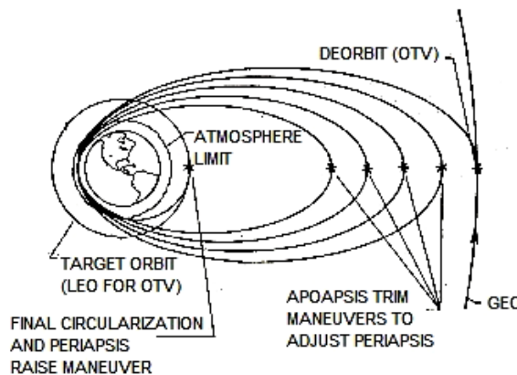
Figure 1. Multipass aerobraking.
