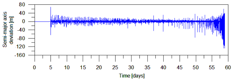
Figure 5. Semi-major axis deviation as function of time.
