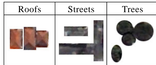
Figure 3: Input Patterns.
