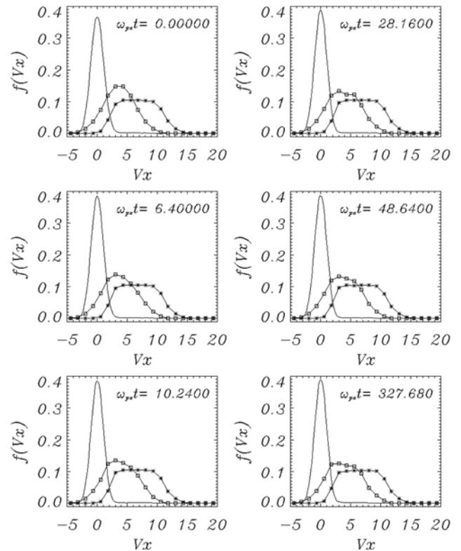
Figure 12. Velocity distribution function for the second case, v_{db2-S} = 0.5v_{db1} . Different times along the simulation are presented. The line with asterisks shows the first beam, and the line with squares shows the second beam.
