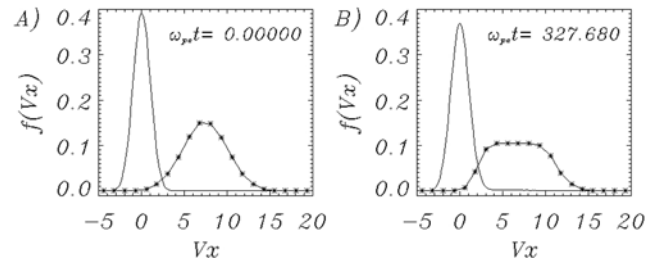
Figure 4. Velocity distribution function for the standard case. (a) Initial time and (b) final time of the simulation are presented. The solid line shows the background plasma, and the line with asterisks shows the first beam.
