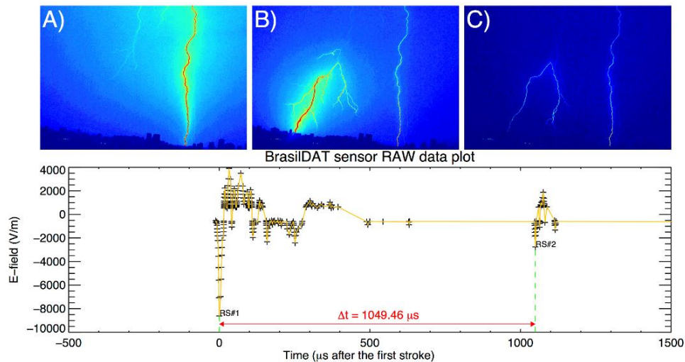
Figure 8 Above: A), B) and C), selected video frames displayed with false color from the blue channel of the colored camera; Below: BrasilDAT waveform of the UI stroke of flash #85.
