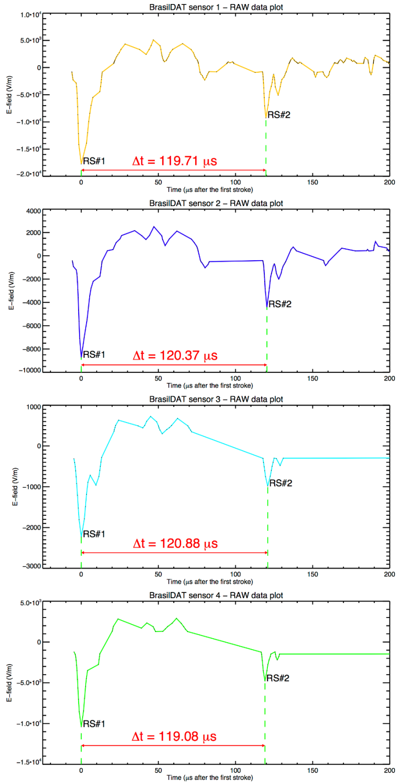
Figure 16 Example of electric field RAW data from four different BrasilDAT sensors for the same forked stroke event.
