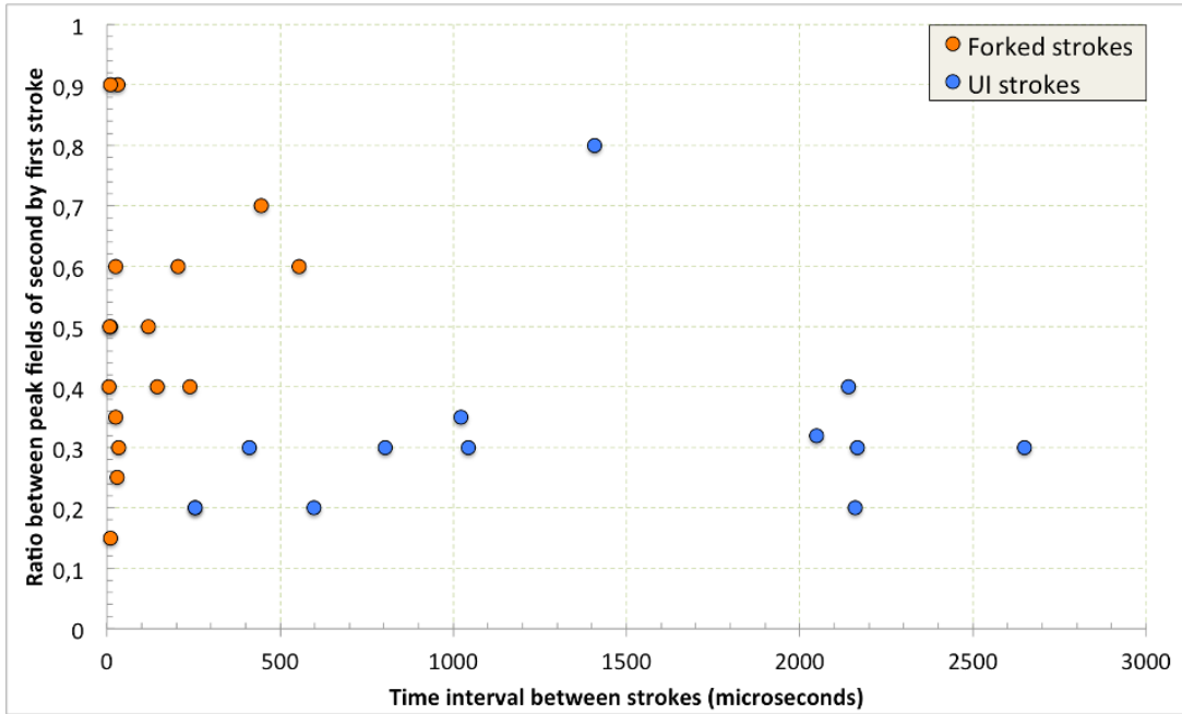
Figure 17 Plot of the ratio between the return stroke electric field peaks of each MGCS event (second over first) versus the time interval between these peaks. Orange circles correspond to forked strokes and blue circles to UI strokes.
