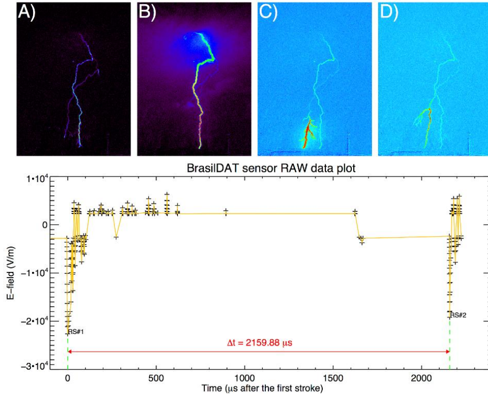
Figure 5 Above: A), B), C) and D), selected video frames displayed with false color from the monochromatic camera; Below: BrasilDAT waveform of the UI stroke of flash #17.
