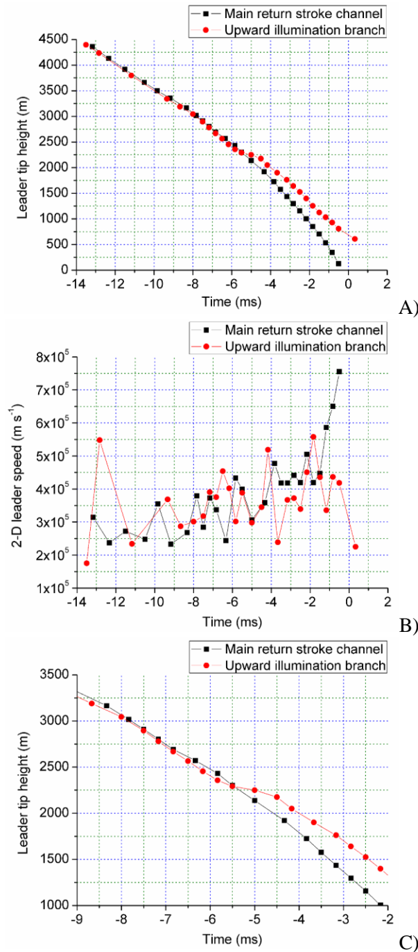
Figure 11 Temporal evolution of A) stepped leader tip height and B) 2-D leader speed of the UI stroke of flash #85. C) is equivalent to A) but zoomed into the instant the leader tips (main and UI) diverged.
