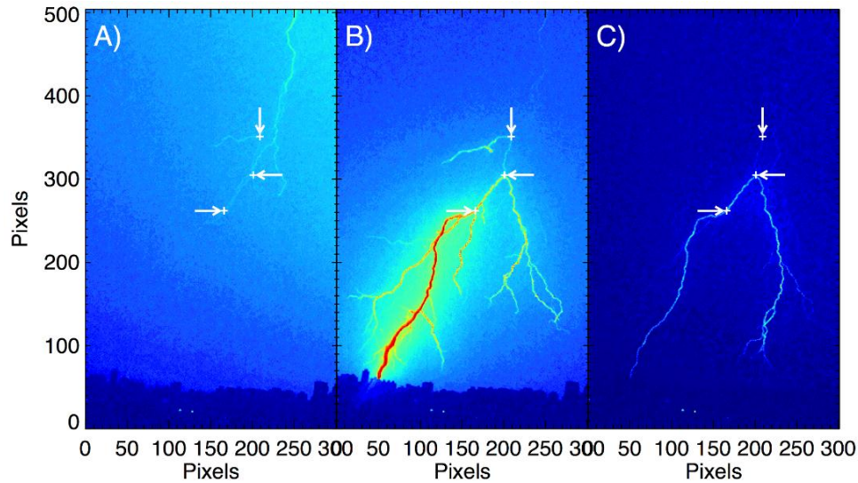
Figure 9 Details of the region of the UI branch of flash #85 (false color from the blue channel data). A) was cut from the main stroke frame, while B) and C) were cut from the first and second frames of the UI process, respectively (three and four frames after the main stroke). Each pixel (vertical or horizontal) is equivalent to approximately 9.3 meters.
