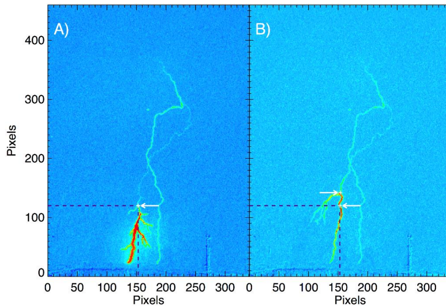
Figure 6 The evolution of the UI process of flash #17 over two consecutive video frames. Each pixel (vertical or horizontal) is equivalent to approximately 20 meters.
