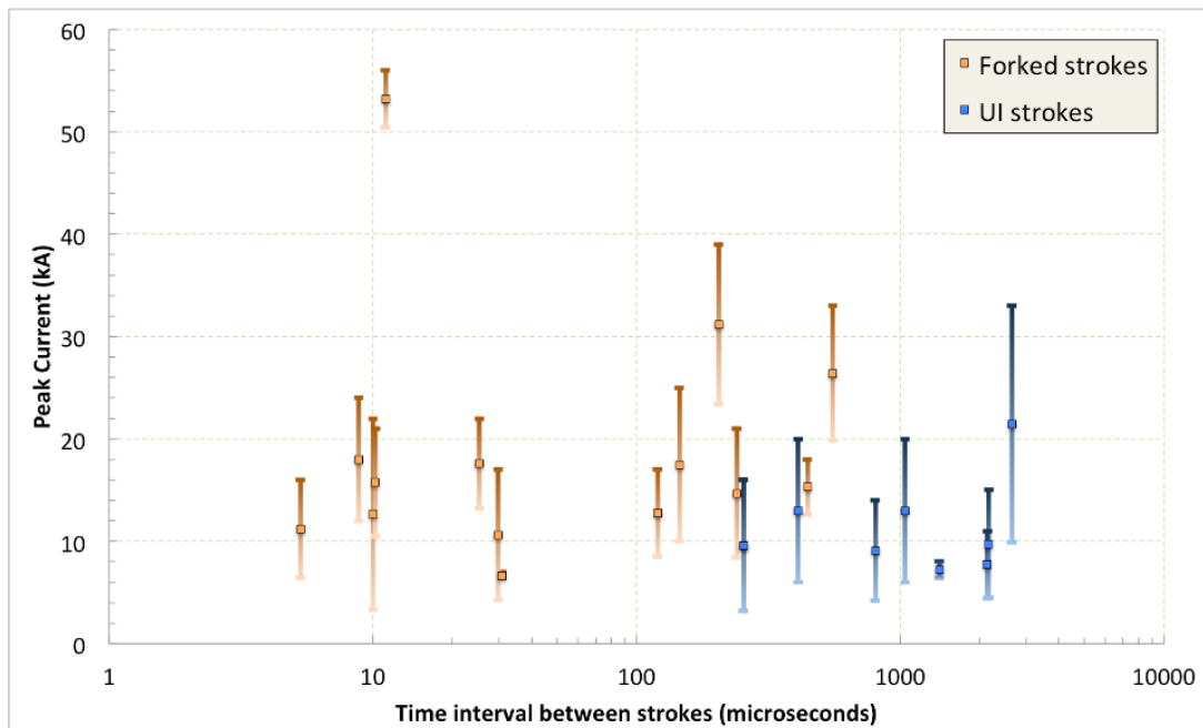
Figure 18 Plot of the peak current estimates of both strokes on each MGCS event versus the time interval between them. The vertical bars represent the first and second strokes in each event. Orange bars correspond to forked strokes and blue bars to UI strokes. The upper limit of the bars are always the peak current of the first stroke and the lower limit the peak current of the second. The horizontal axis is presented in a logarithm scale in order to favor the visualization of the results.
