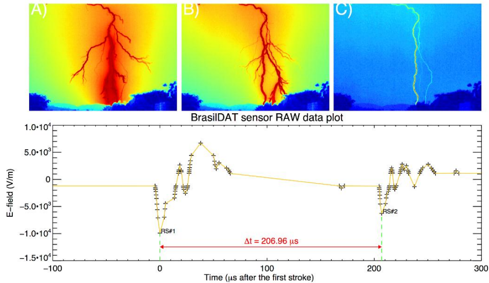
Figure 4 Above: A), B) and C), selected video frames displayed with false color from the monochromatic camera; Below: BrasilDAT waveform of the forked stroke of flash #54.
