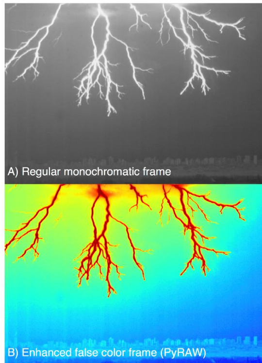
Figure 2 A) One frame selected from a high-speed video recorded by a monochromatic Phantom V9.1 camera; B) the same frame enhanced through the PyRAW library functionalities using a rainbow color palette.
