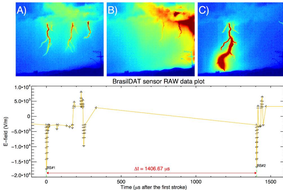
Figure 12 Above: A), B) and C), selected video frames displayed with false color from the red channel of the colored camera; Below: BrasilDAT waveform of the UI stroke of flash #22.
