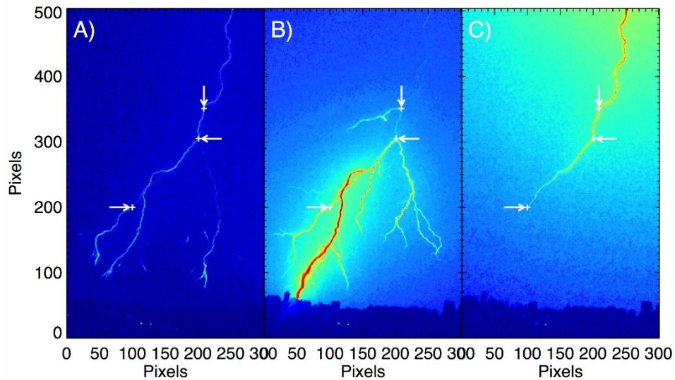
Figure 10 Details of A) the stepped leader, B) the UI process and C) the subsequent attempted leader that occurs after the UI of flash #85. All frames are false color from the blue channel data of the colored camera. Each pixel (vertical or horizontal) is equivalent to approximately 9.3 meters.
