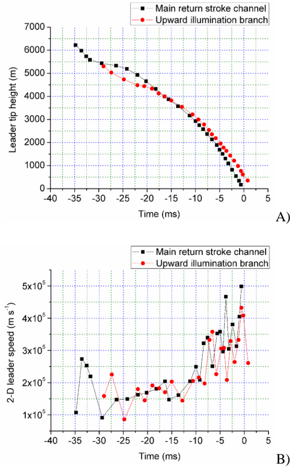
Figure 7 Temporal evolution of A) stepped leader tip height and B) 2-D leader speed of the UI stroke of flash #17.
