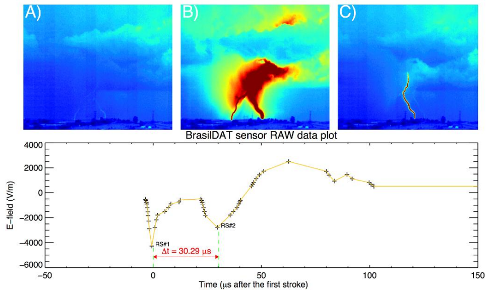
Figure 3 Above: A), B) and C), selected video frames displayed with false color from the monochromatic camera; Below: BrasilDAT waveform of the forked stroke of flash #1.
