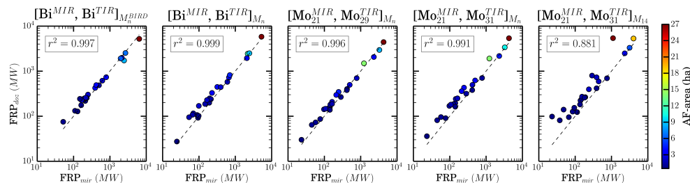
Figure 14. Comparison between \text{FRP}_{\text{mir}} and \text{FRP}_{\text{doz}} for the 5[ \text{sensor}_{\text{band}}^{\text{MIR}}, \text{sensor}_{\text{band}}^{\text{TIR}} ] _{\text{mask}} selection introduced in the text. The masks ( M_n , M_n^{\text{BIRD}} , and M_{14} ) are different approaches to evaluate fire and background radiance (see Appendix B for more details). \text{FRP}_{\text{mir}} is retrieved following the approach of Wooster et al. (2005) and \text{FRP}_{\text{doz}} is directly calculated from the output of the Dozier (1981) algorithm assuming the fire is behaving as a black body.
