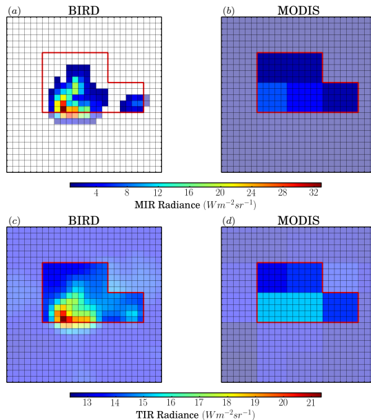
Figure 13. Geo-referenced, co-located imagery collected by (a) and (c) the BIRD satellites 185 m spatial resolution Hotspot Recognition Sensor (HSRS) in the MIR and LWIR bands respectively (Zhukov et al., 2006), and (b) and (d) the 1 km spatial resolution data collected in the MIR and TIR bands of the MODIS sensor operated on the Terra satellite (Giglio et al., 2003). Data are from a Siberian forest fire observed on the 10 July 2003 (57.8873° N; 97.7711° E). See Appendix B for full wavelength specifications of each sensor. Imaging times were 05:32 UTC for BIRD, and 04:55 UTC for MODIS. The red outline shows the fire cluster contour derived from the active fire pixels detected by the Collection 5 MODIS Active Fire and Thermal Anomaly product of (Giglio et al., 2003). In the BIRD imagery, the MIR band only shows pixels detected as fire, while in the TIR band pixels outside the MODIS cluster mask are shaded.
