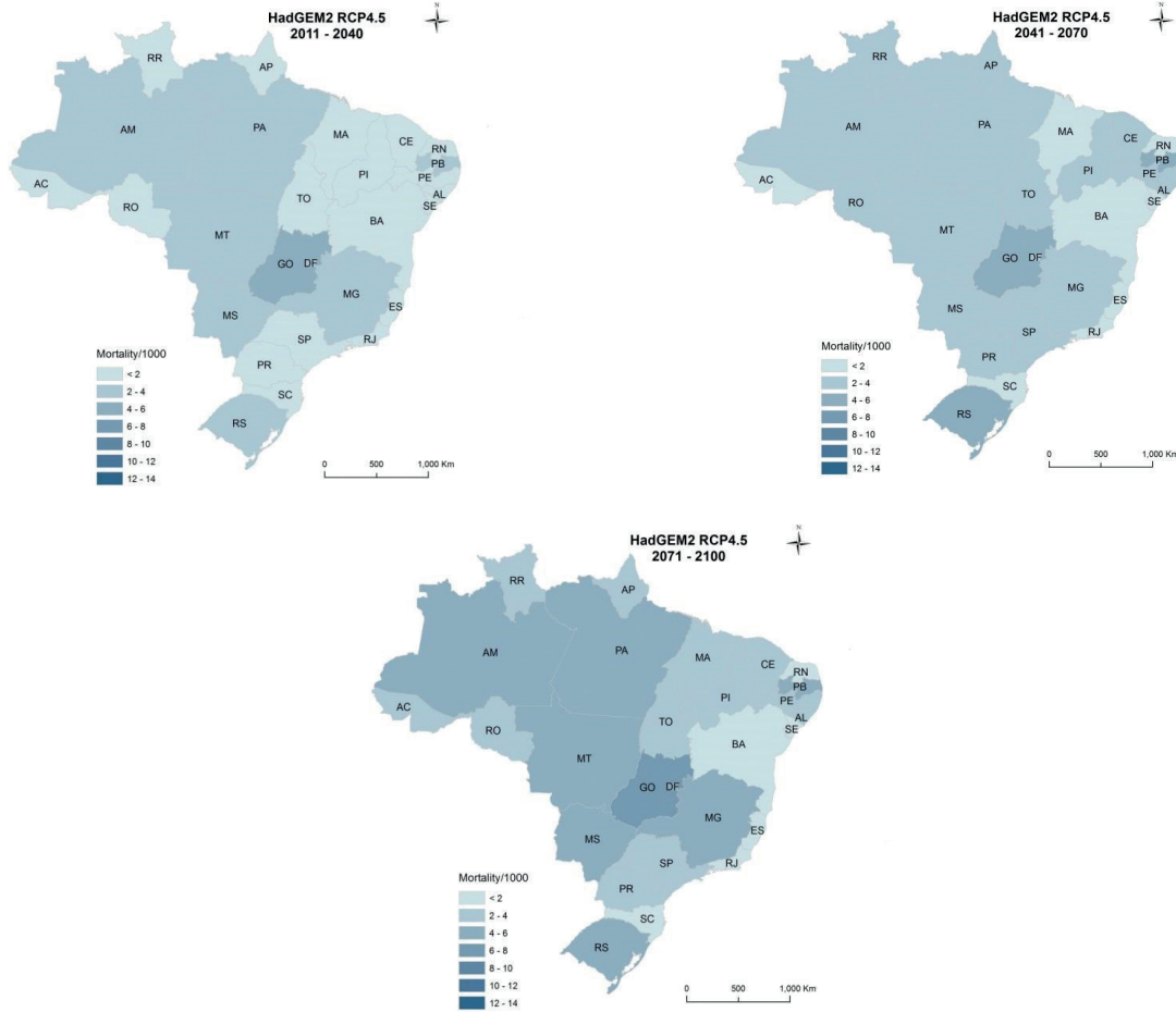
Premature mortality rates for projections of the Eta-HadGEM2-ES model RCP 4.5 scenario
