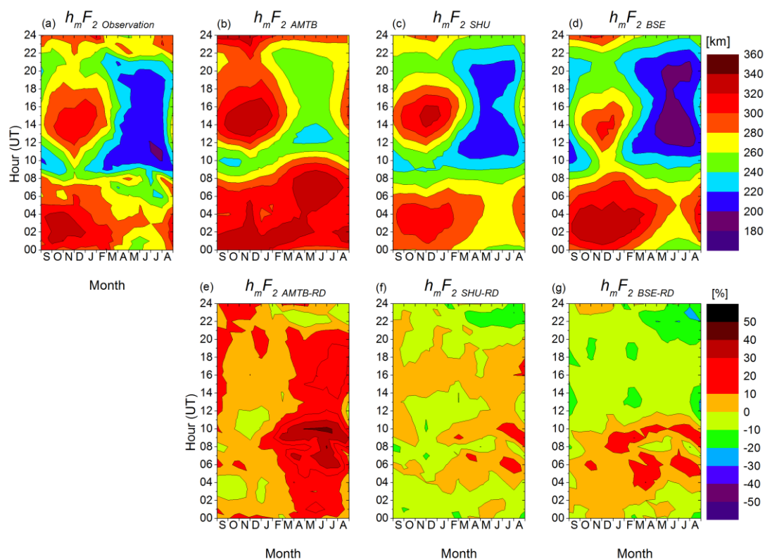
Fig. 3: Contour plot of the monthly averaged h_m F_2 (a) measured by the Santa Maria Digisonde (SMK29), provided by (b) AMTB, (c) SHU, and (d) BSE coefficients. The respective Relative Deviation (RD) in percent is placed in the lower panels for (e) AMTB, (f) SHU, and (g) BSE.
