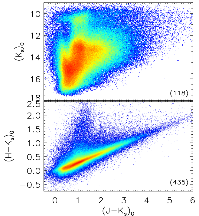
Figure 13. (J - K)_0 versus (K)_0 colour–magnitude diagram (upper panel) and (H - K)_0 versus (J - K)_0 colour–colour diagram (lower panel). The higher number of sources per pixel is shown in the right corner in each diagram. We should probably note that the brightest sources with K_s < 11 mag are saturated.
