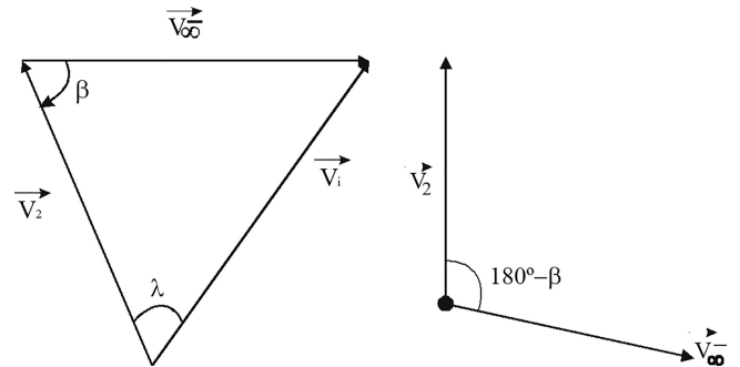
Figura 8: Soma vetorial envolvida no swing-by .
