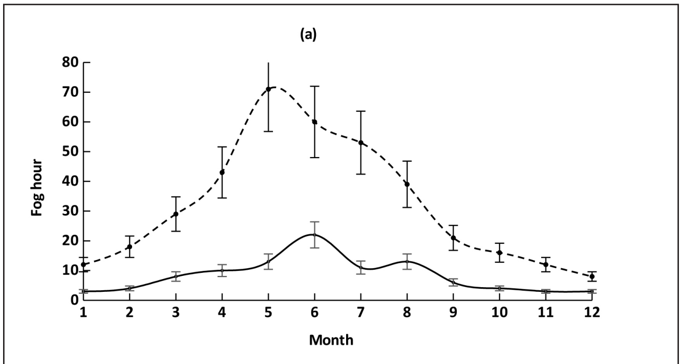
Figure 5 : the average, minimum, maximum monthly fog hours for the periods corresponding to 1961-1990 (dash line) and 1991-2015 (solid line).
